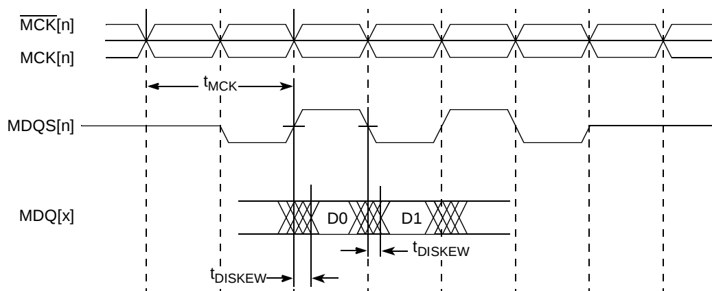
Figure 3. DDR SDRAM Input Timing Diagram ( t_{\text{DISKEW}} )
