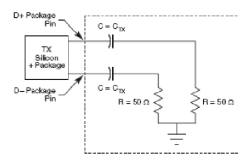
Figure 32. SGMII AC Test/Measurement Load
