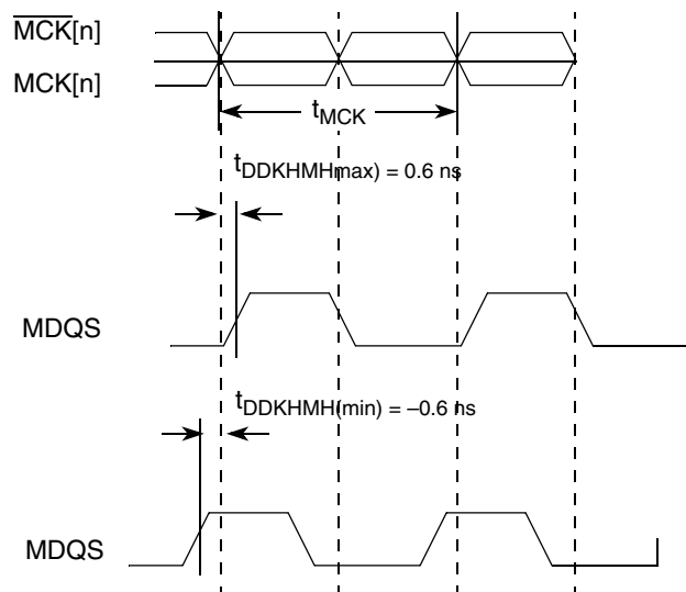
Figure 9. Timing Diagram for t_{\text{DDKHMH}}
