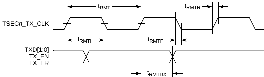
Figure 18. RMI Transmit AC Timing Diagram
