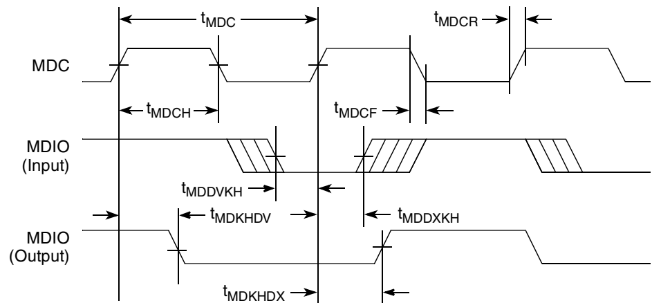
Figure 15. MII Management Interface Timing Diagram
