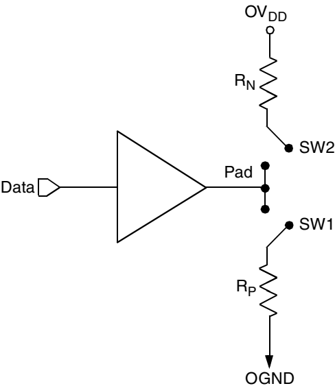
Figure 59. Driver Impedance Measurement
