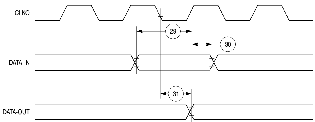
Figure 45. Parallel I/O Data-In/Data-Out Timing Diagram
