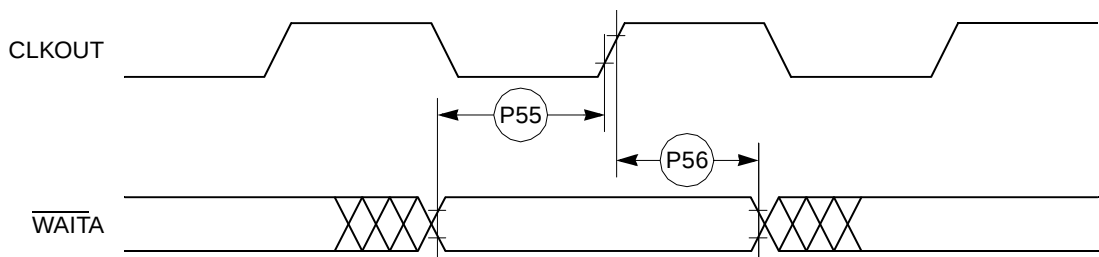
Figure 29. PCMCIA \overline{WAIT} Signals Detection Timing
