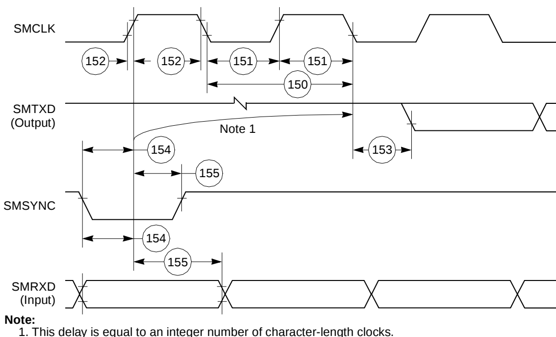
Figure 59. SMC Transparent Timing Diagram
