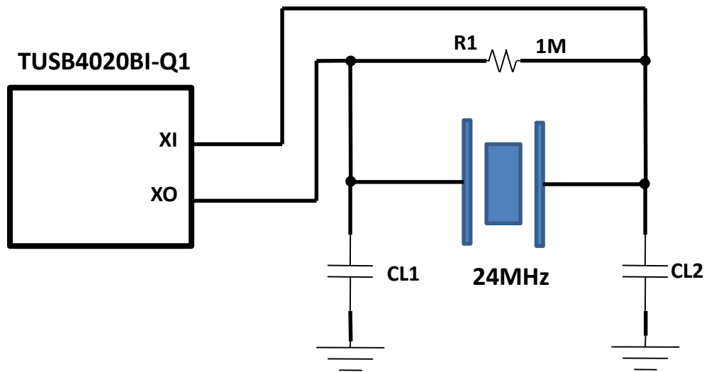
Figure 2. TUSB4020BI-Q1 Clock
