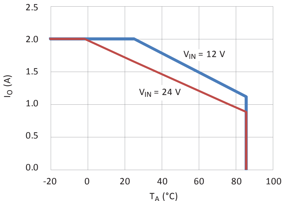
Figure 2. MPM80 thermal derating curve; measurement conditions: V_O = 5\text{ V} , no heatsink
