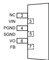
Pin-out Diagram
