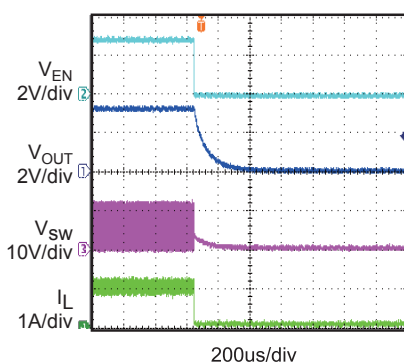
Shut down I_{OUT}
