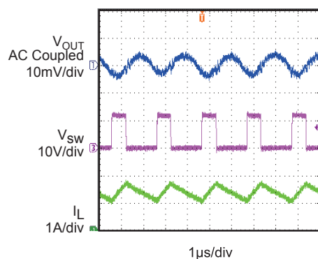
Output Voltage Ripple I_{OUT}=1A
