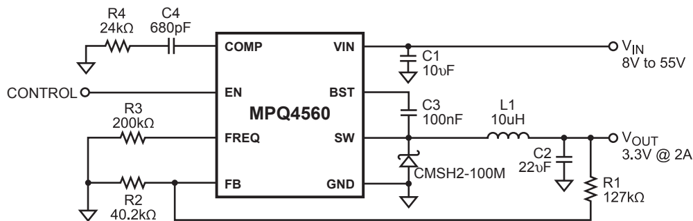
MPQ4560 Typical Application Circuit
