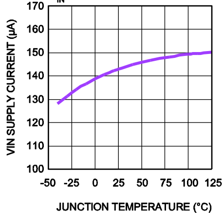
V_{IN} Quiescent Current vs. Junction Temperature
