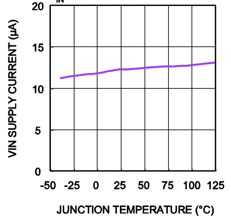
Shutdown Current vs. Junction Temperature
