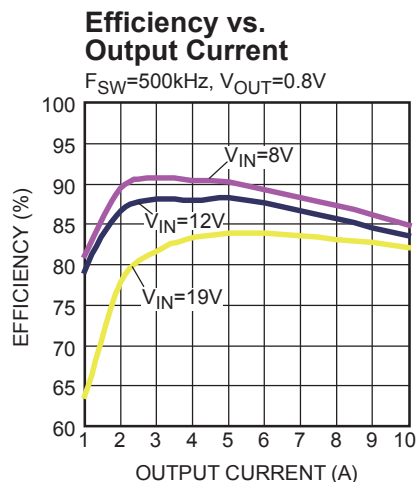
Figure 21 — Efficiency Curve
