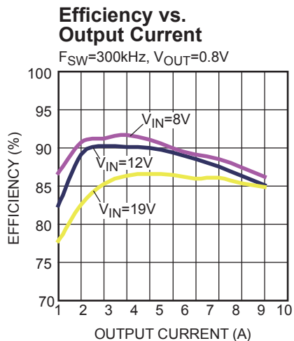
Figure 19 — Efficiency Curve
