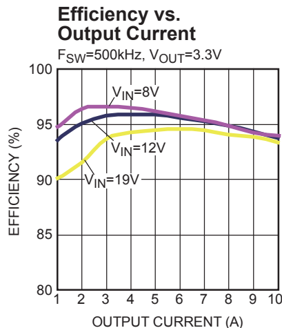
Figure 43 — Efficiency Curve
