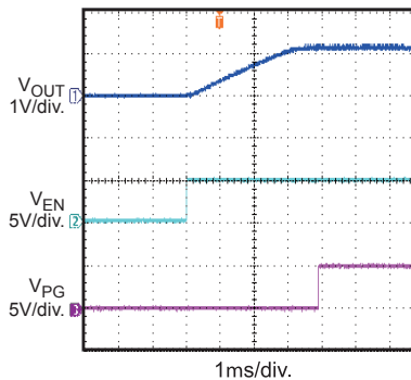
Power Good Through EN
