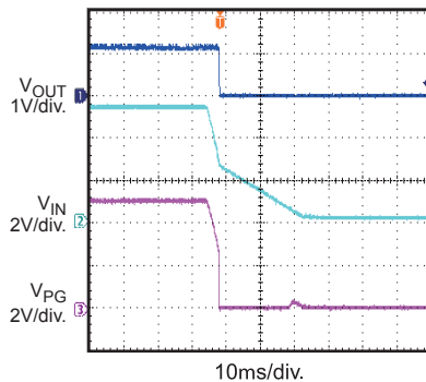
Power Good Through Vin
