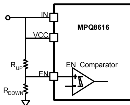
Figure 6—Adjustable UVLO
