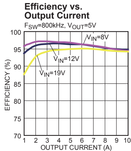
Figure 17 — Efficiency Curve
