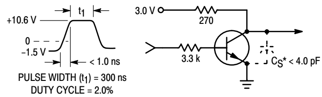
Figure 1. t_{on} Circuit
