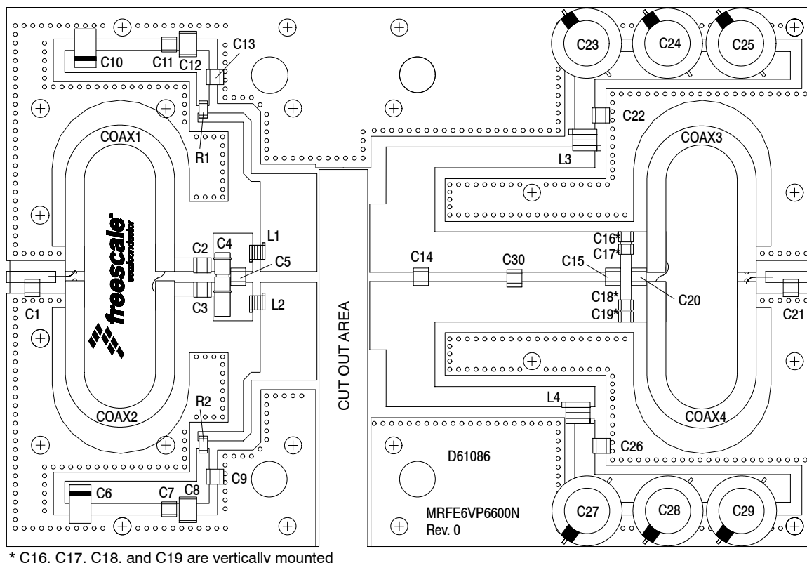
Figure 8. MRFE6VP6600N Narrowband Test Circuit Component Layout — 230 MHz
