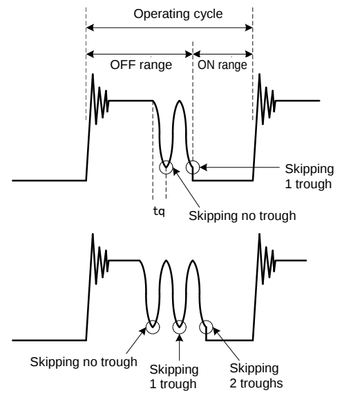
Switching waveform model
