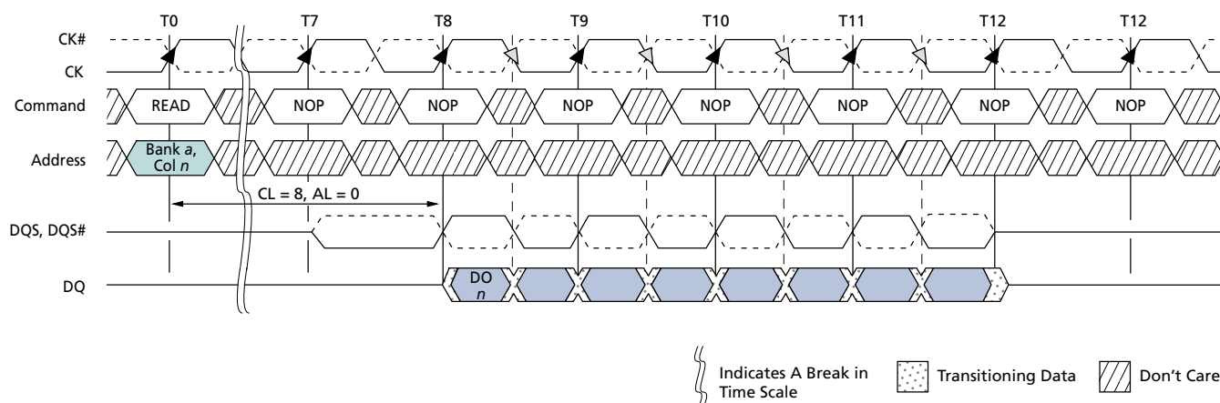
Figure 68: READ Latency
