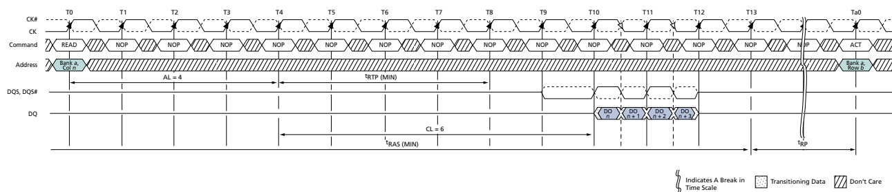
Figure 77: READ with Auto Precharge (AL = 4, CL = 6)
