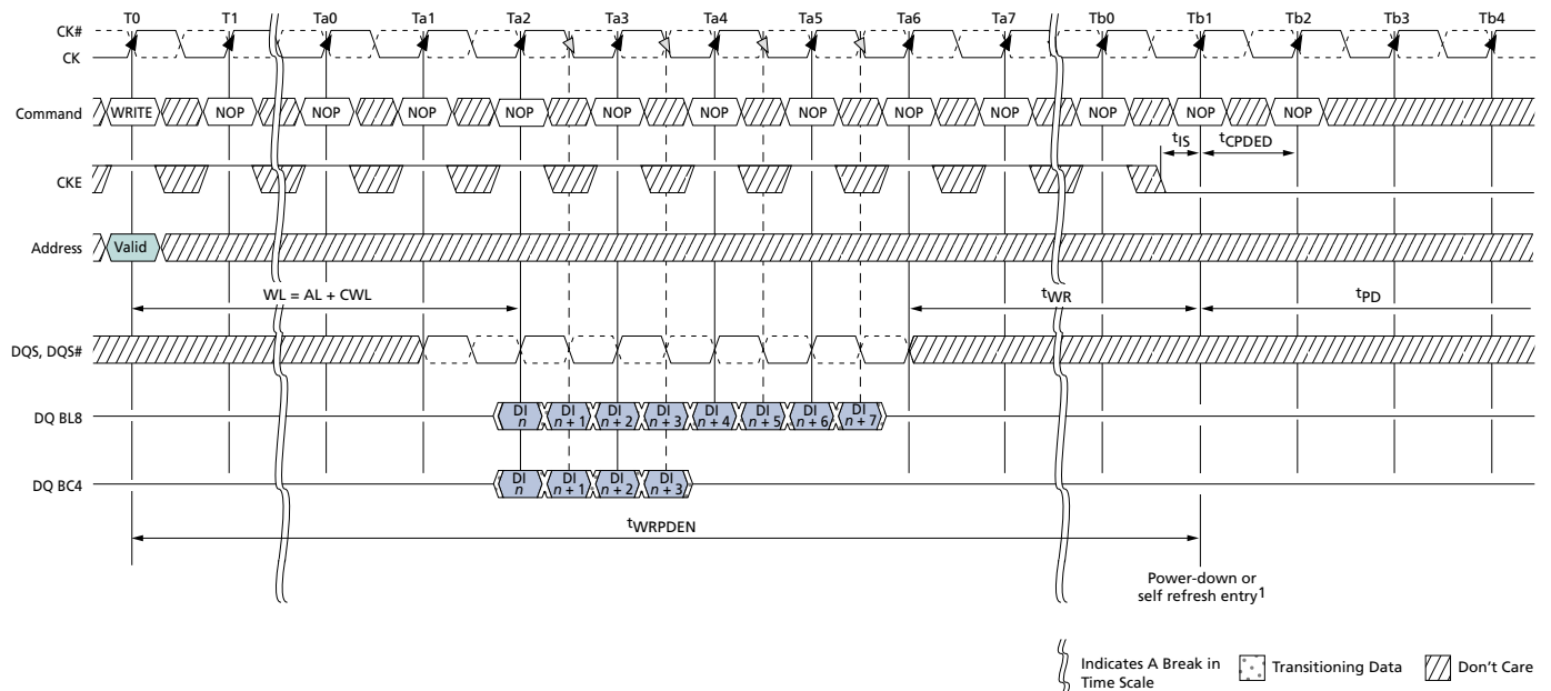
Figure 101: Power-Down Entry After WRITE
