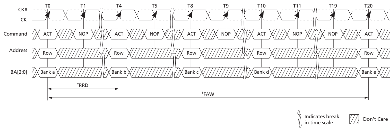
Figure 64: Example: t_{FAW}
