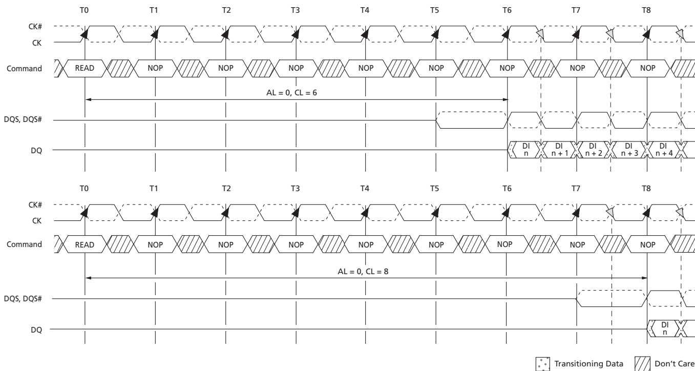
Figure 51: READ Latency
