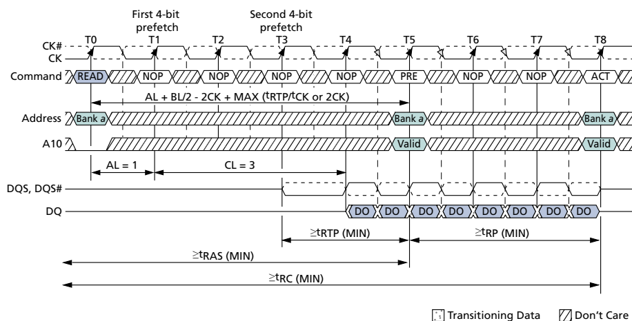
Figure 52: READ-to-PRECHARGE – BL = 8
