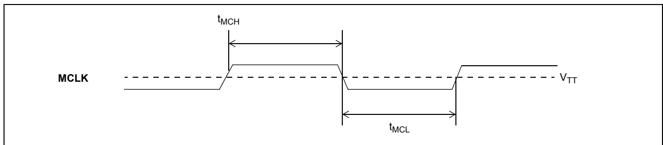
Figure 12 - Master Clock
