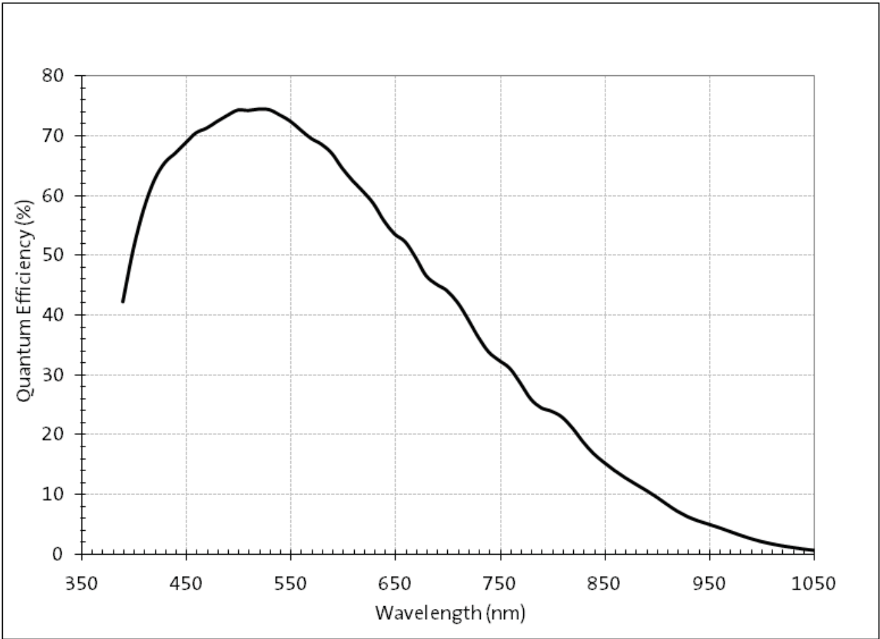
Figure 27: Estimated Quantum Efficiency – Monochrome Sensor
