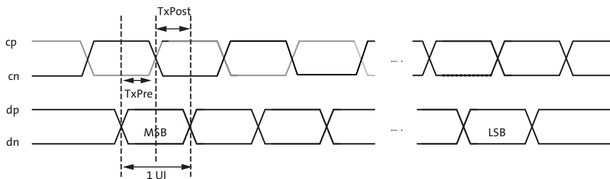
Figure 12: Timing Diagram
