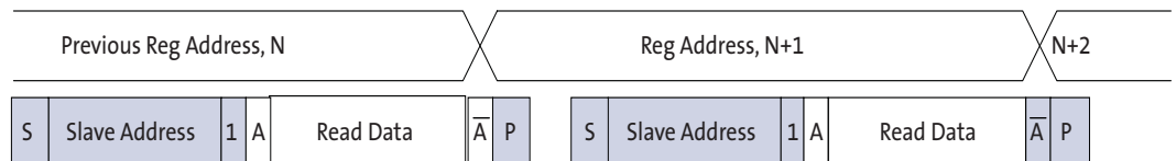
Figure 21: Single READ from Current Location
