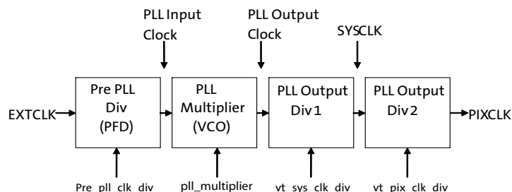
Figure 15: PLL-Generated Master Clock PLL Setup
