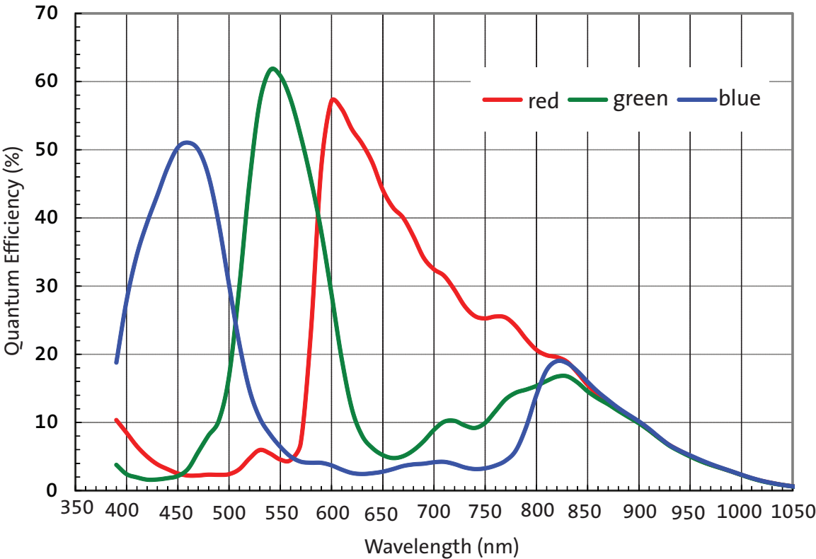
Figure 24: Quantum Efficiency – Color Sensor
