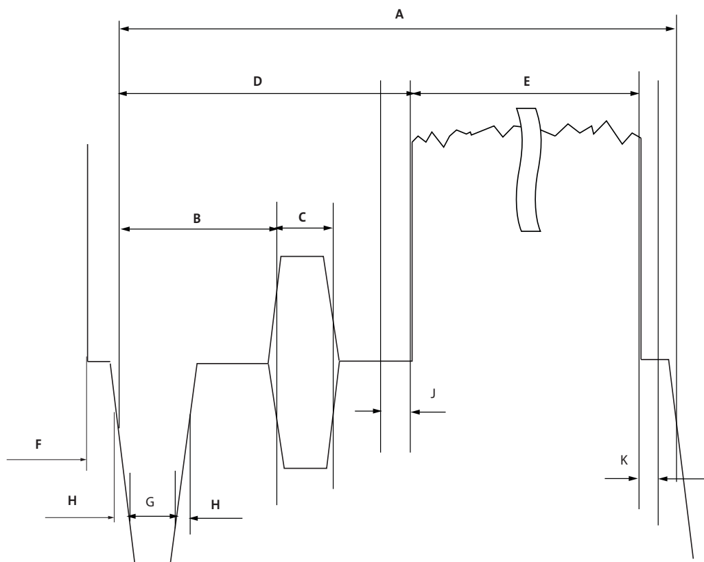
Figure 56: Video Timing
