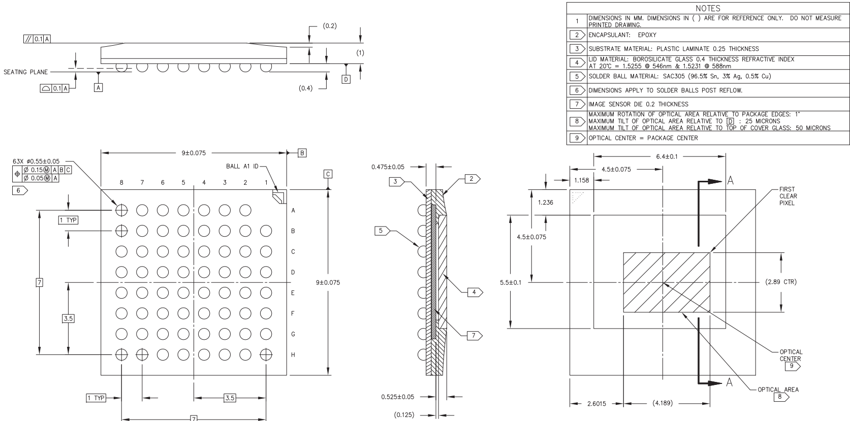
Figure 61: 63-Ball iBGA Package Outline Drawing
