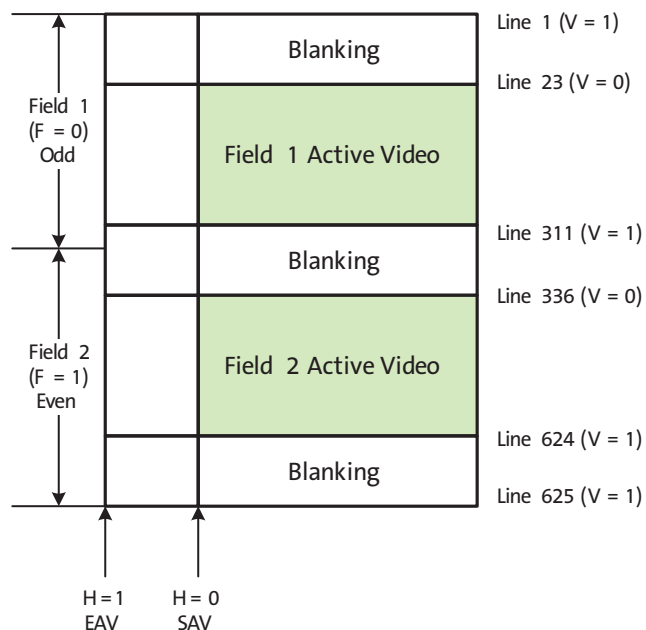
Figure 40: Typical CCIR656 Vertical Blanking Intervals for 625/50 Video System
