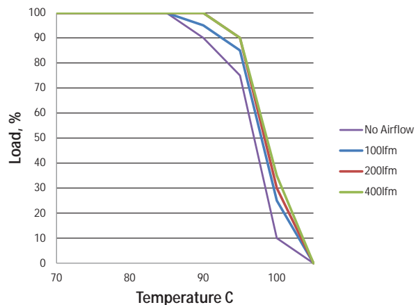
MTC2S2405MC- 36Vin
