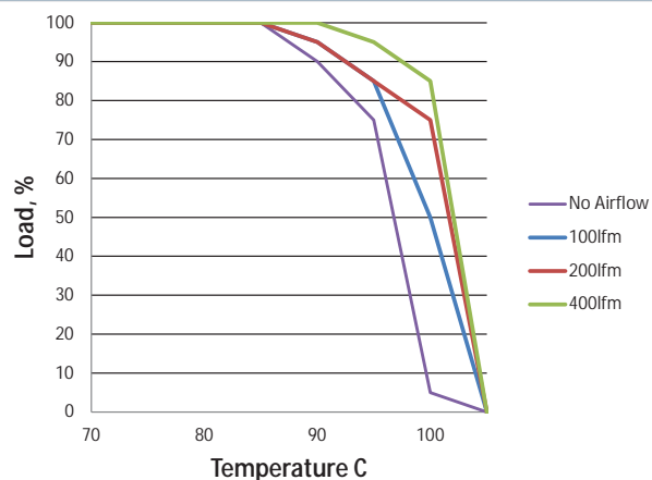
MTC2S1212MC- 18Vin
