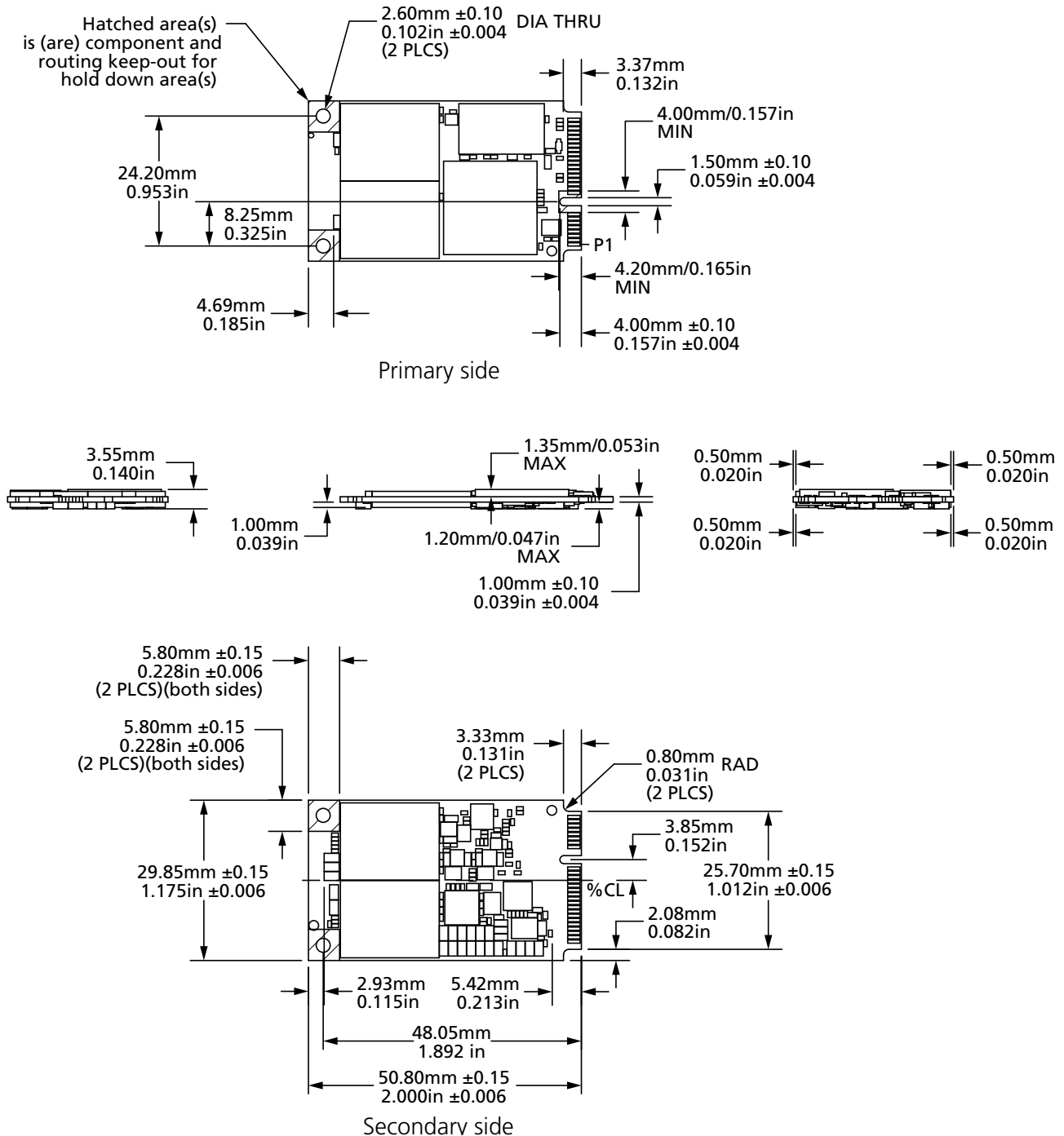
Figure 5: mSATA Package
