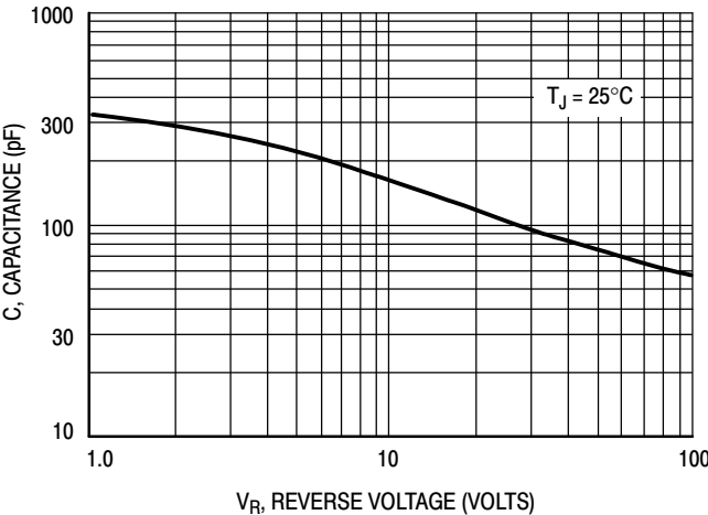
Figure 10. Typical Capacitance
