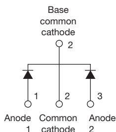
VS-MURB1620CT-1PbF
