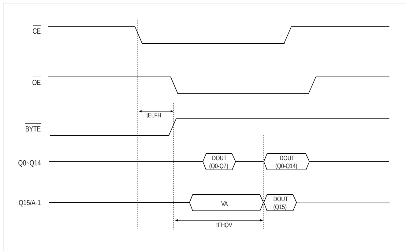
Figure 25. BYTE TIMING WAVEFORM FOR READ OPERATIONS (BYTE switching from byte mode to word mode)
