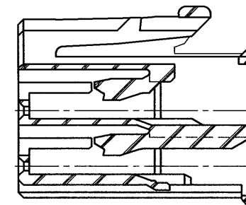
SECT. B-B
