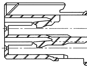
SECT. A-A
