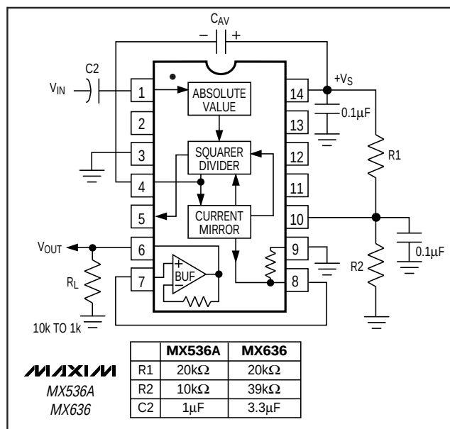
Figure 5. Single-Supply Operation
