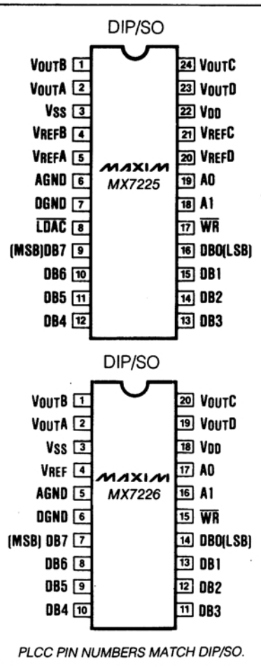
Pin Configurations
