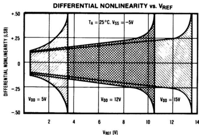
Typical Operating Characteristics
