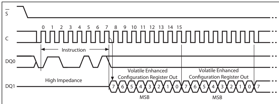
Figure 41. Read Volatile Enhanced Configuration Register instruction sequence
