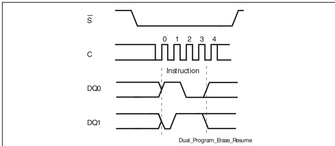
Figure 57. Program/Erase Resume instruction sequence DIO-SPI
