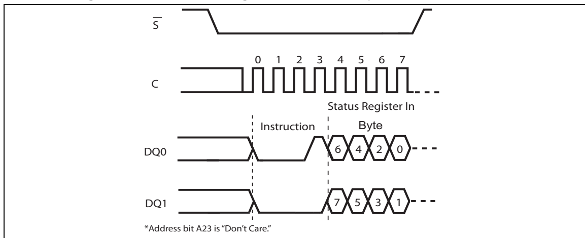
Figure 59. Write Status Register instruction sequence DIO-SPI
