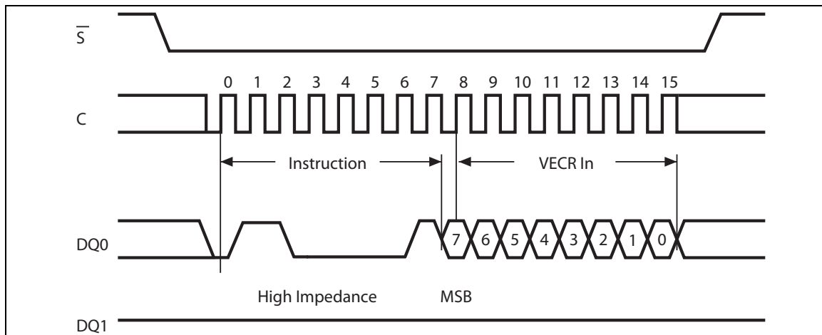
Figure 42. Write Volatile Enhanced Configuration Register instruction sequence
