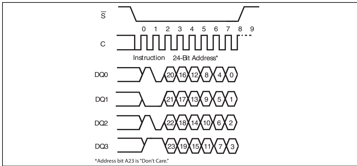
Figure 83. Sector Erase instruction sequence QIO-SPI
