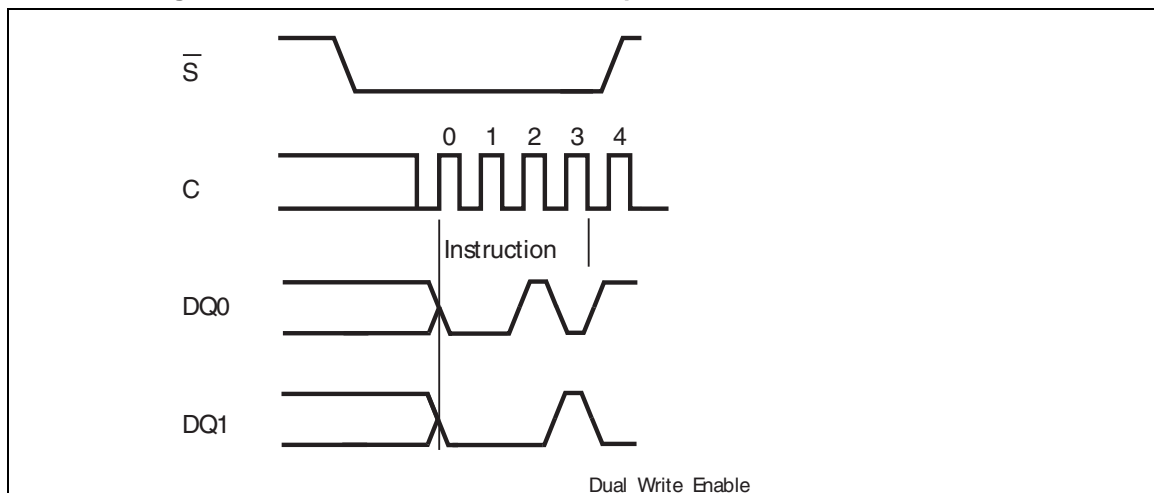
Figure 47. Write Enable instruction sequence DIO-SPI
