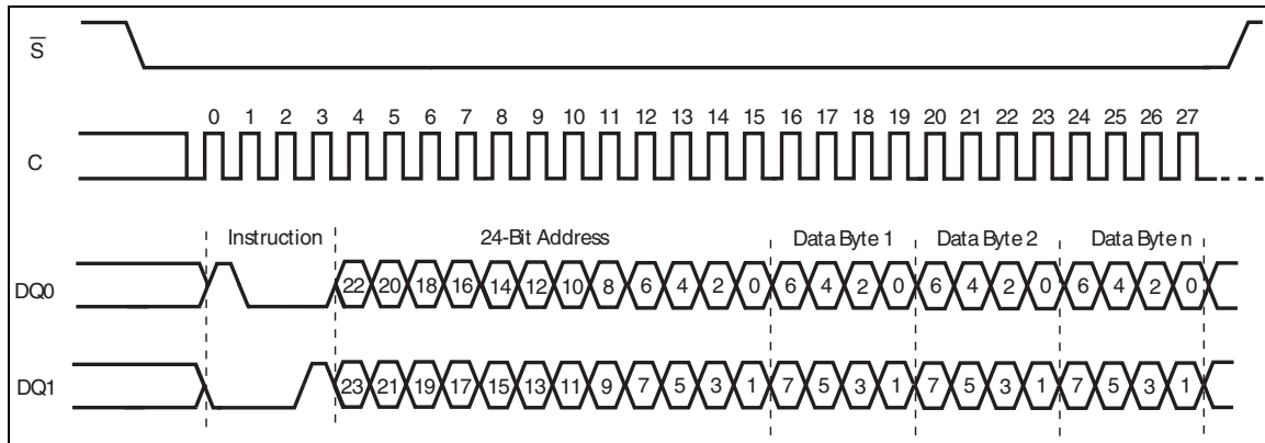
Figure 52. Program OTP instruction sequence DIO-SPI
