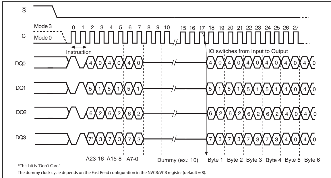
Figure 71. Quad Read Serial Flash Discovery Parameter
