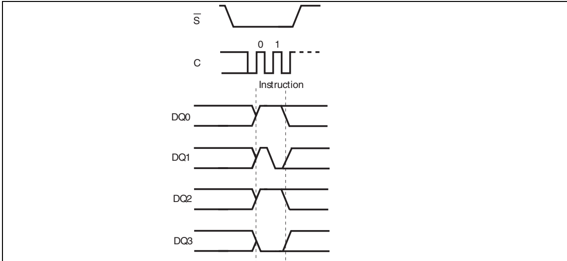
Figure 85. Program/Erase Suspend instruction sequence QIO-SPI
