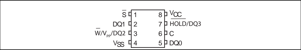
Figure 2. SO8N, SO8W and MLP8 connections
