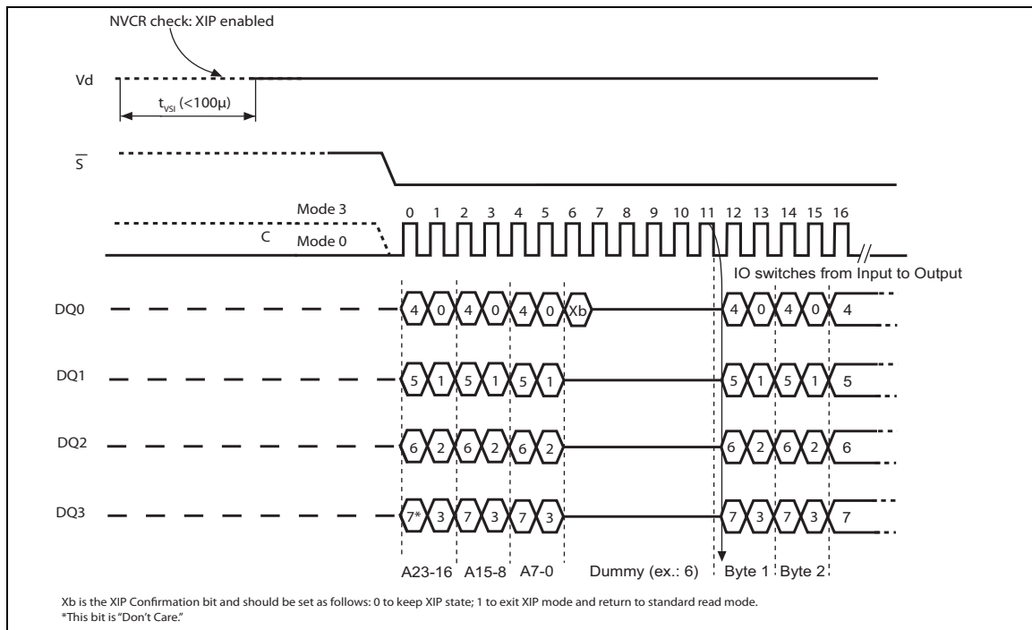
Figure 100. XIP mode directly after power on
