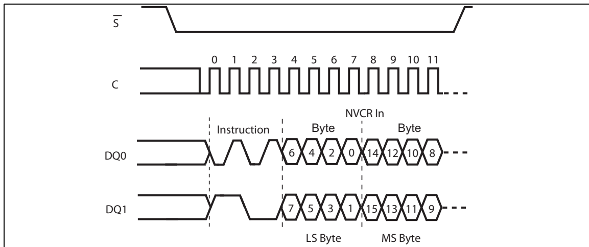
Figure 65. Write NV Configuration Register instruction sequence DIO-SPI
