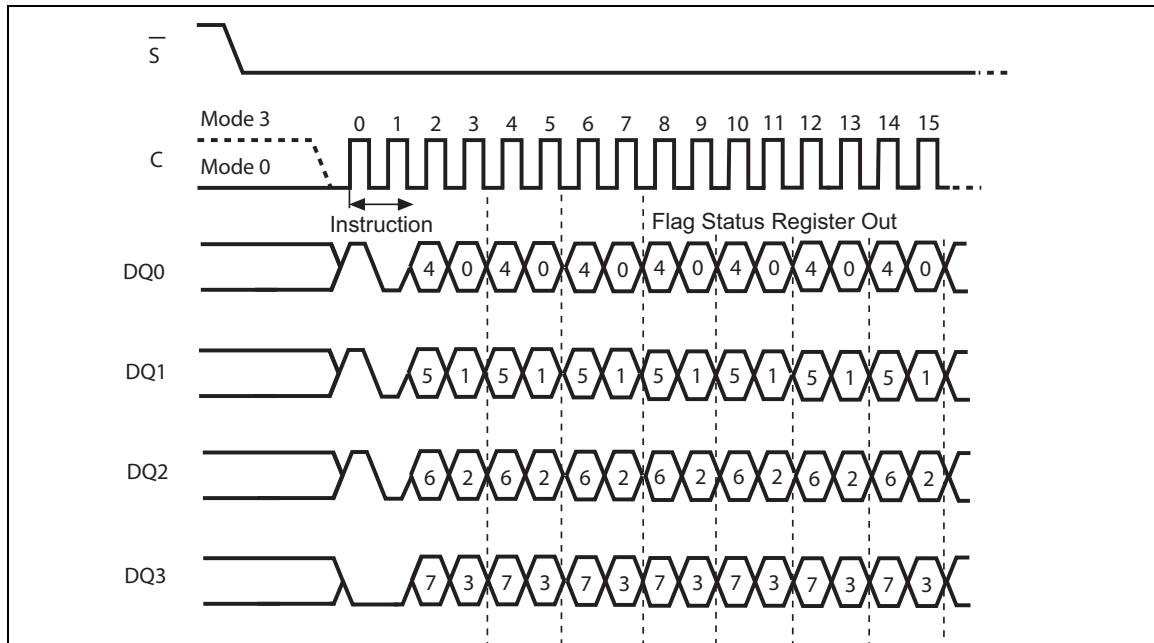
Figure 91. Read Flag Status Register instruction sequence QIO-SPI
