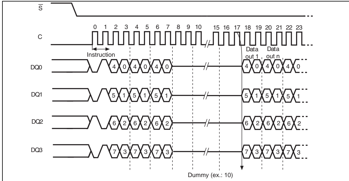
Figure 75. Read OTP instruction and data-out sequence QIO-SPI
