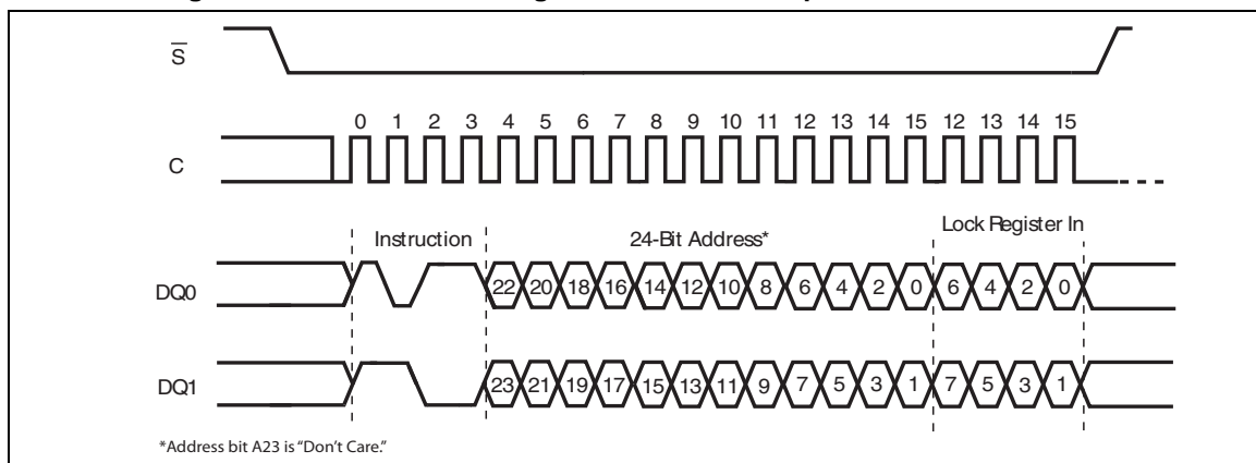
Figure 61. Write to Lock Register instruction sequence DIO-SPI
