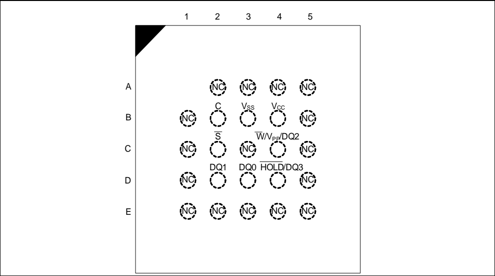
Figure 4. BGA connections
