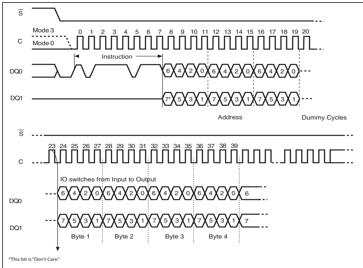
Figure 15. Dual I/O Fast Read instruction sequence
