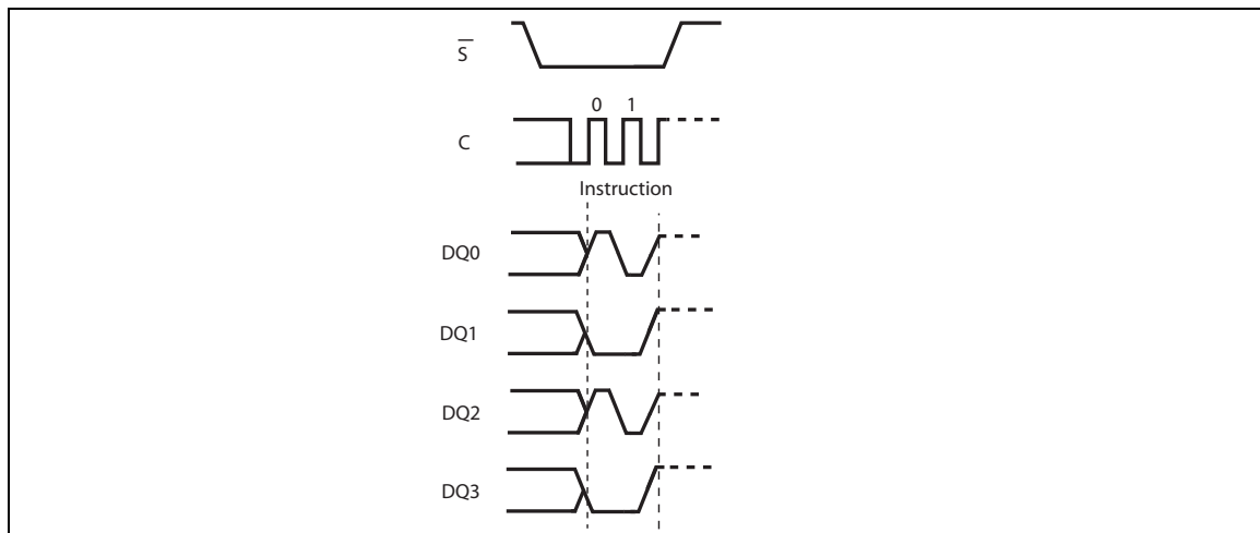
Figure 92. Clear Flag Status Register instruction sequence QIO-SPI
