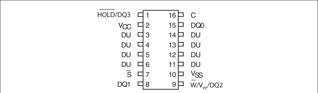
Figure 3. SO16 connections
