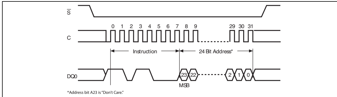
Figure 29. Sector Erase instruction sequence
