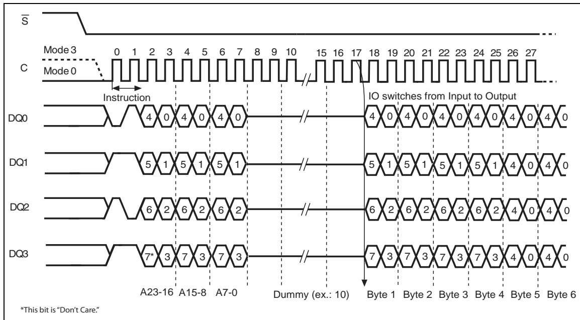
Figure 74. Quad Command Fast Read instruction and data-out sequence QIO-SPI, EBh
