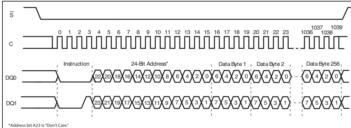
Figure 49. Dual Command Page Program instruction sequence DIO-SPI, 02h
