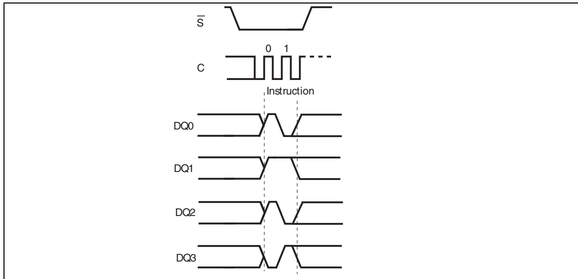
Figure 86. Program/Erase Resume instruction sequence QIO-SPI
