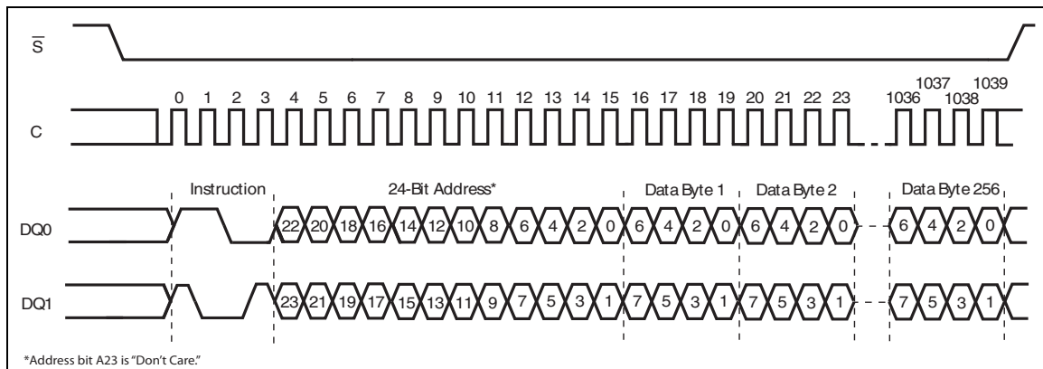
Figure 51. Dual Command Page Program instruction sequence DIO-SPI, D2h
