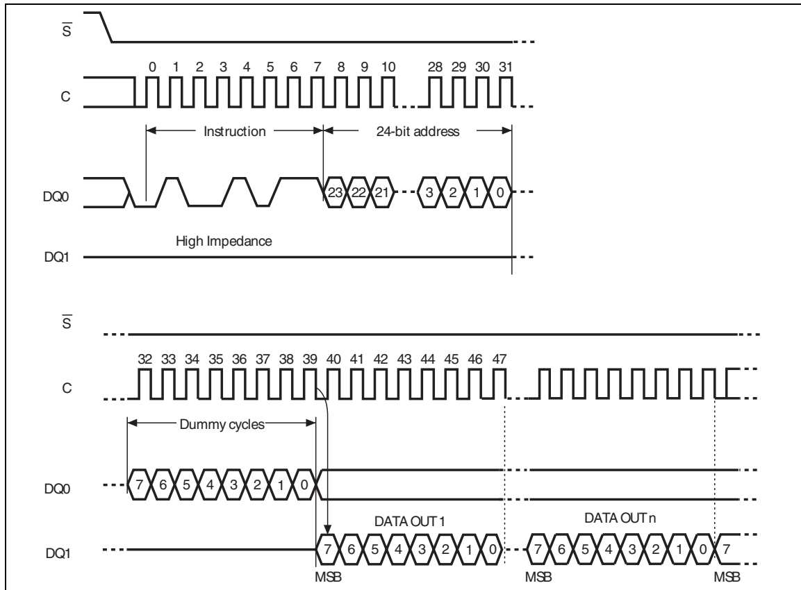
Figure 18. Read OTP instruction and data-out sequence
