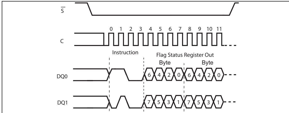
Figure 62. Read Flag Status Register instruction sequence DIO-SPI
