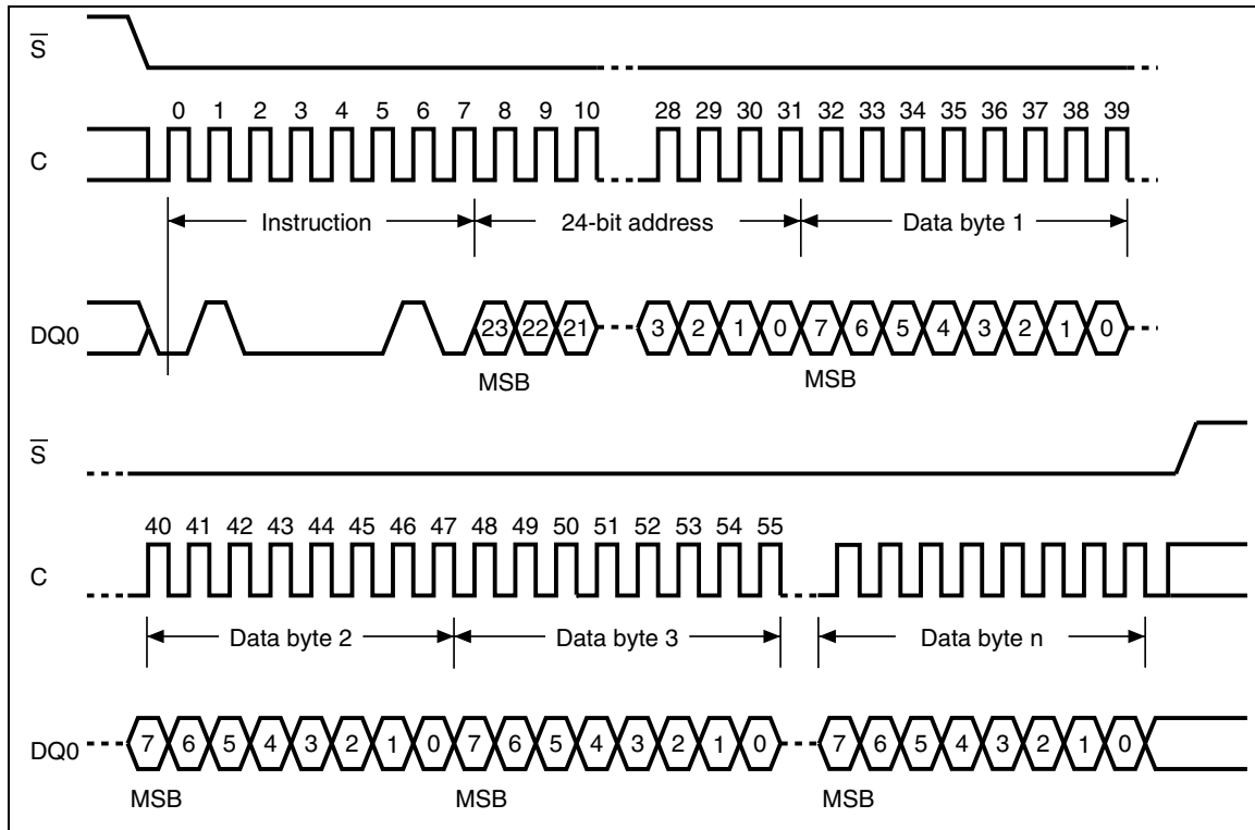
Figure 26. Program OTP instruction sequence
