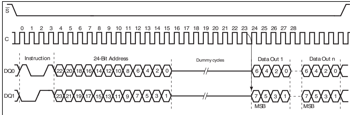
Figure 46. Read OTP instruction and data-out sequence DIO-SPI
