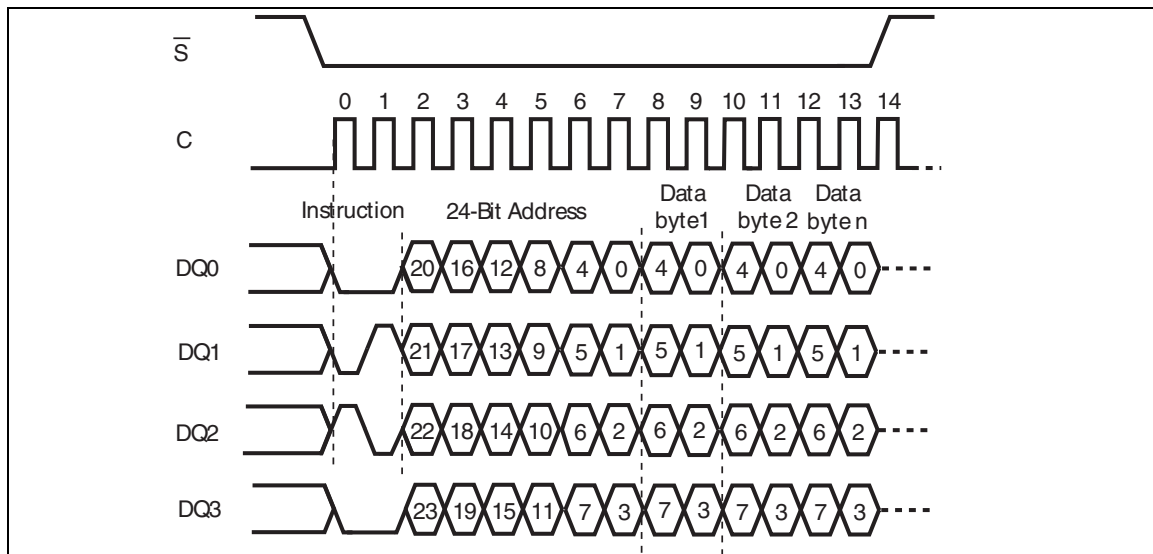
Figure 81. Program OTP instruction sequence QIO-SPI
