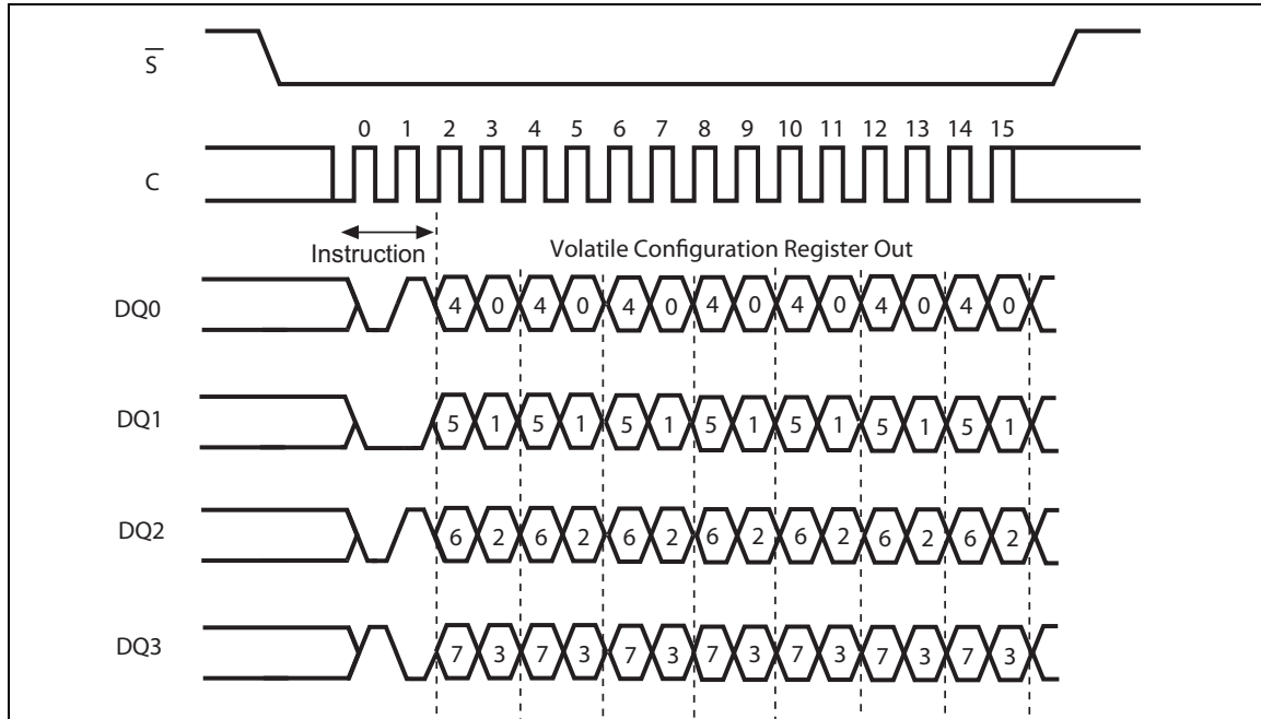
Figure 95. Read Volatile Configuration Register instruction sequence QIO-SPI
