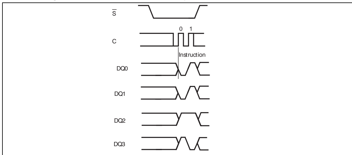
Figure 84. Bulk Erase instruction sequence QIO-SPI
