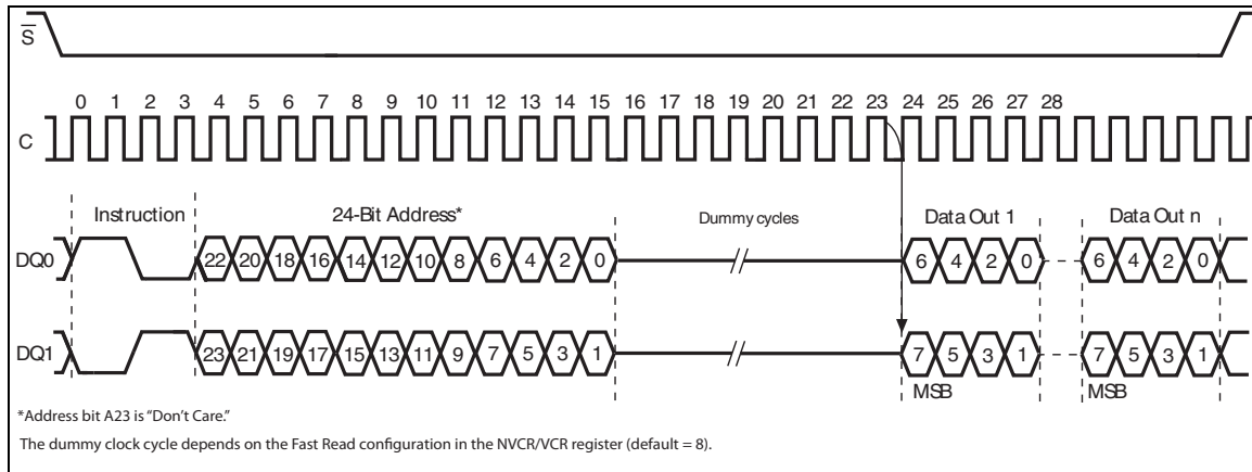
Figure 44. Dual Read Serial Flash Discovery Parameter
