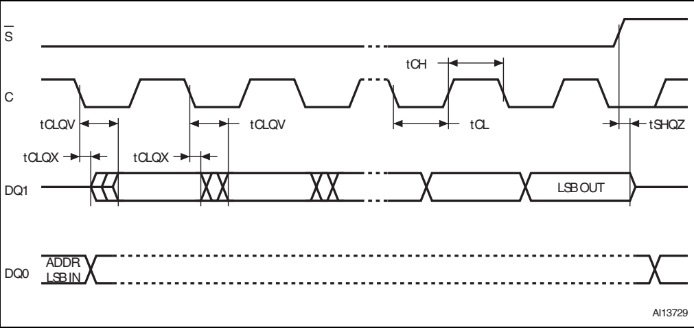
Figure 108. Output timing
