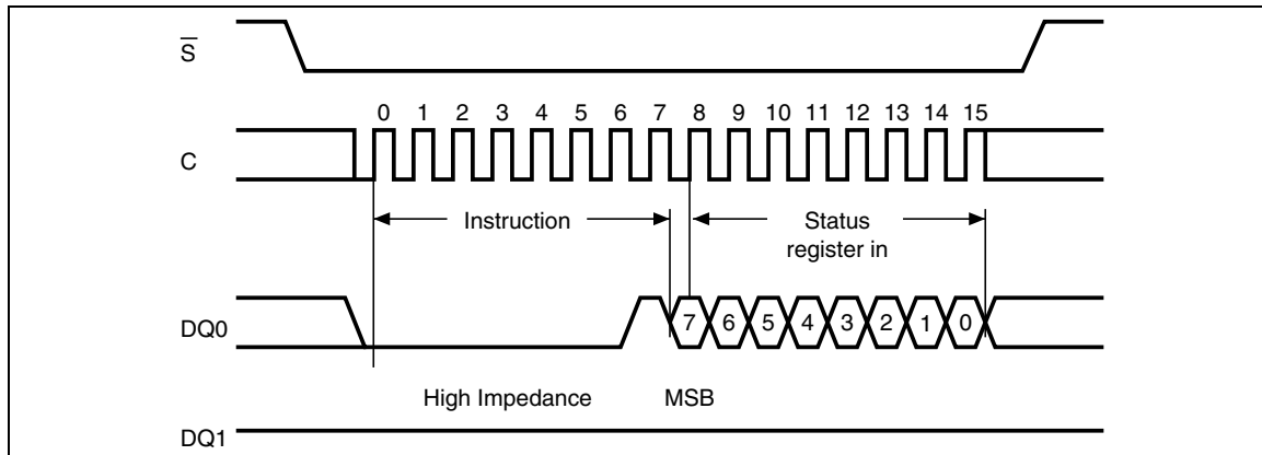
Figure 32. Write Status Register instruction sequence
