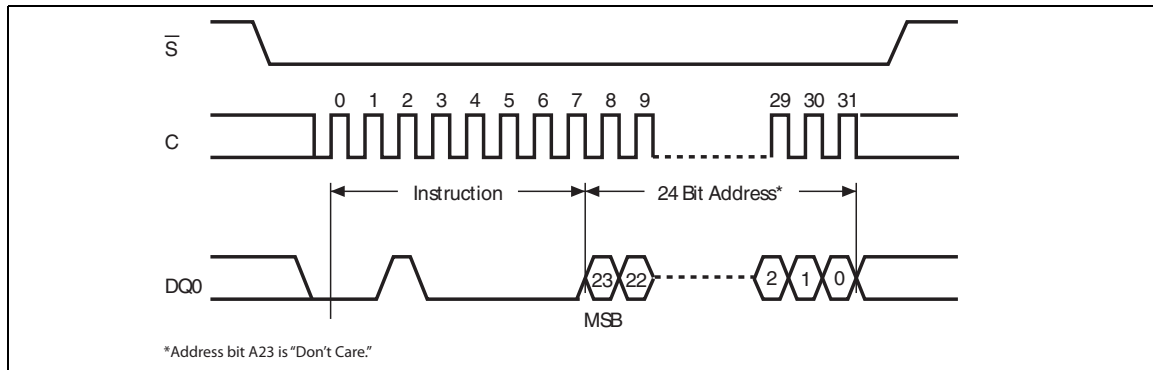
Figure 28. Subsector Erase instruction sequence
