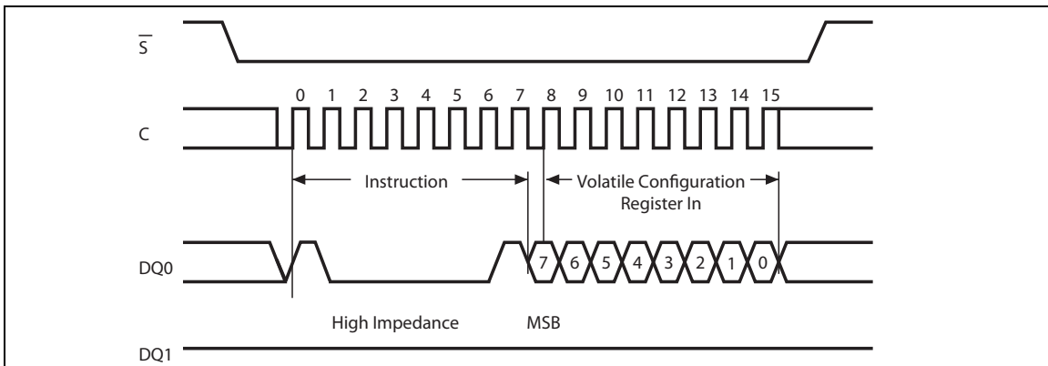
Figure 40. Write Volatile Configuration Register instruction sequence
