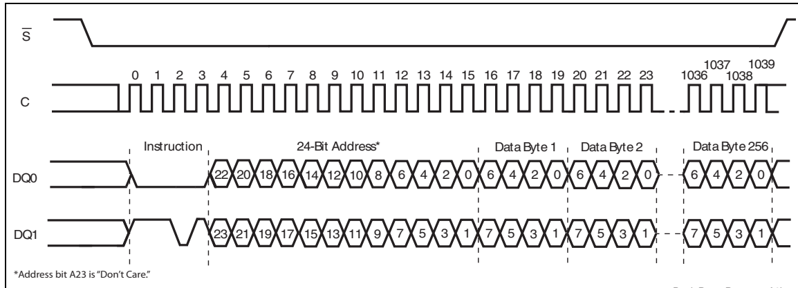
Figure 51. Dual Command Page Program instruction sequence DIO-SPI, D2h
