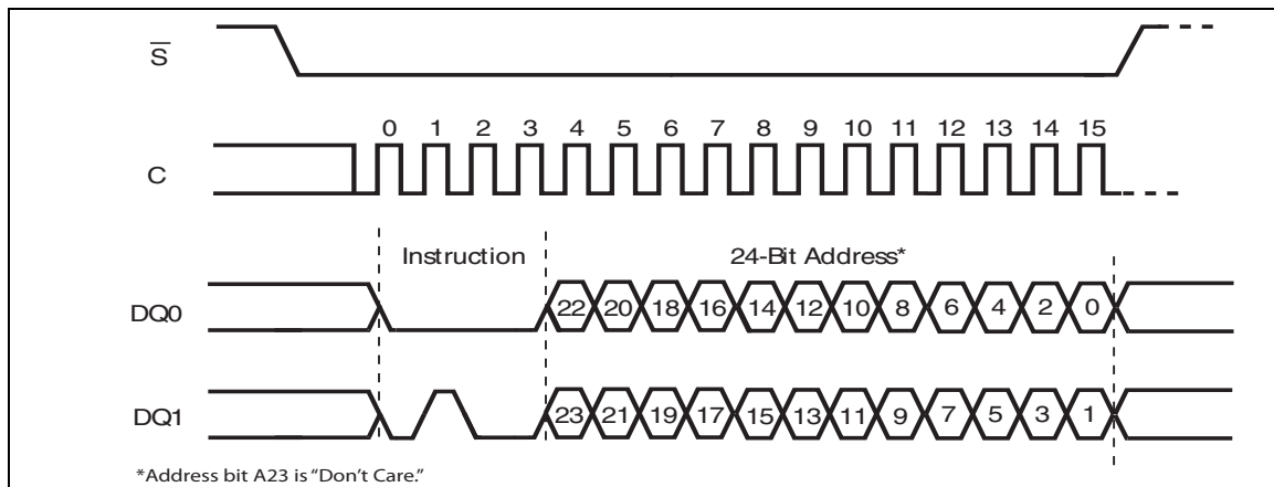
Figure 53. Subsector Erase instruction sequence DIO-SPI
