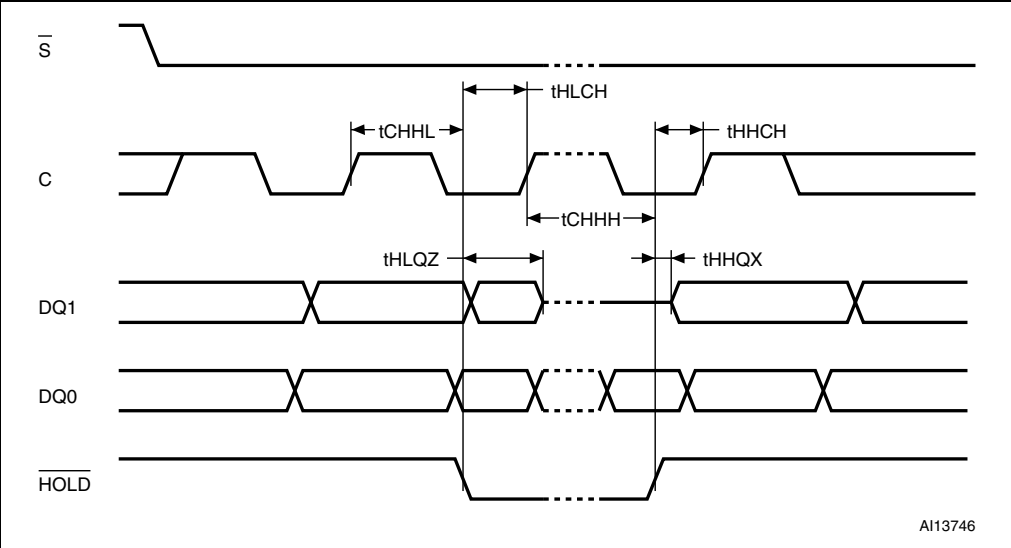
Figure 107. Hold timing
