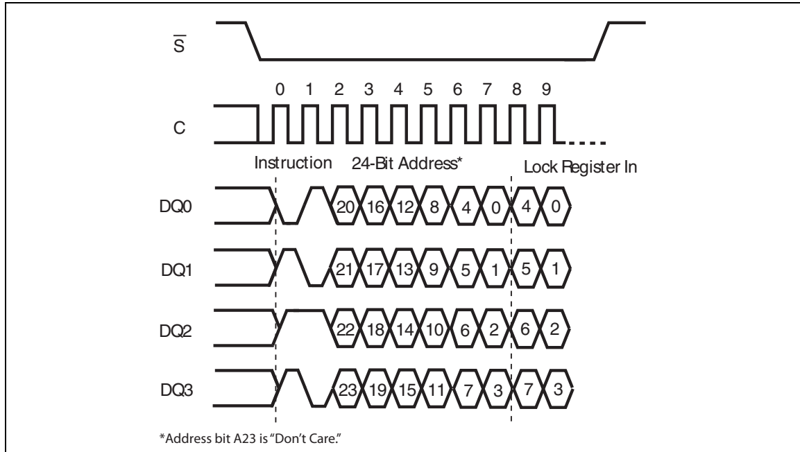
Figure 90. Write to Lock Register instruction sequence QIO-SPI
