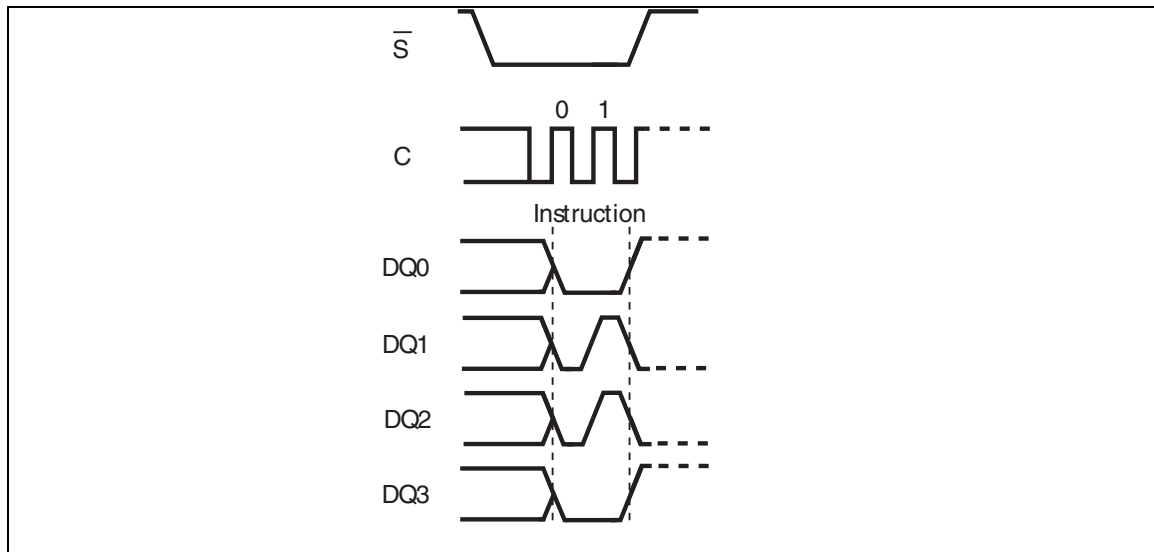
Figure 76. Write Enable instruction sequence QIO-SPI
