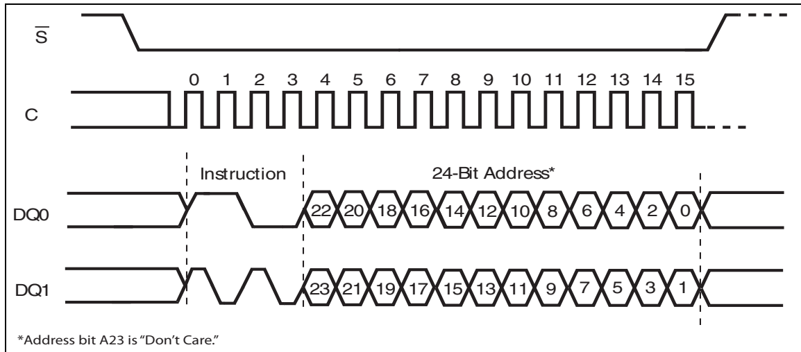
Figure 54. Sector Erase instruction sequence DIO-SPI
