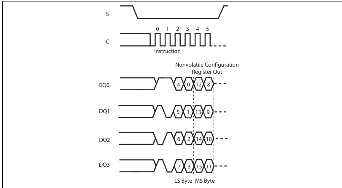
Figure 93. Read NV Configuration Register instruction sequence QIO-SPI
