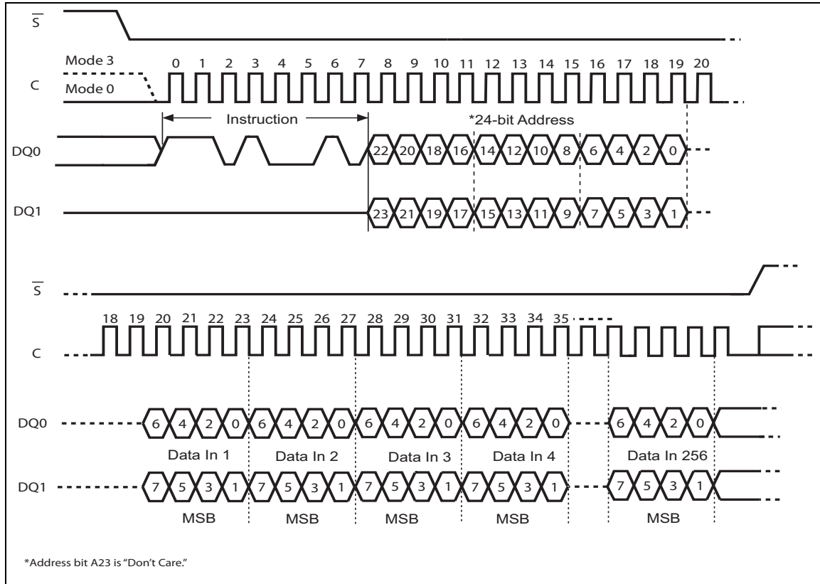
Figure 23. Dual Input Extended Fast Program instruction sequence
