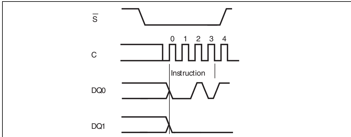
Figure 48. Write Disable instruction sequence DIO-SPI
