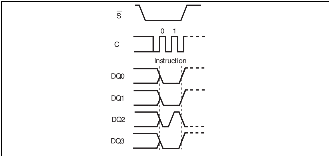
Figure 77. Write Disable instruction sequence QIO-SPI
