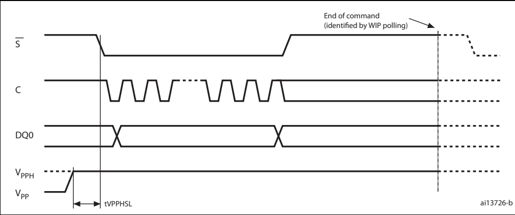
Figure 109. VPP H timing
