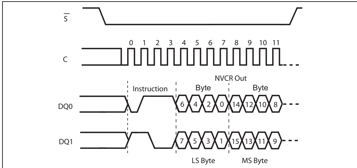
Figure 64. Read NV Configuration Register instruction sequence DIO-SPI
