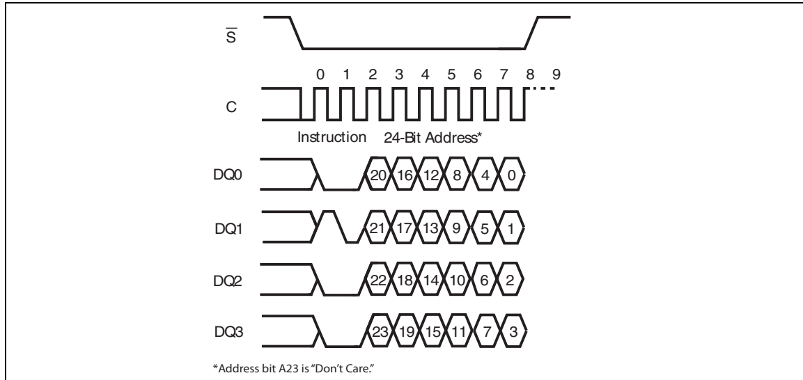
Figure 82. Subsector Erase instruction sequence QIO-SPI
