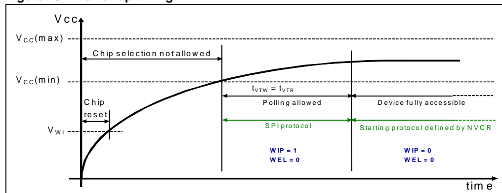
Figure 102. Power-up timing
