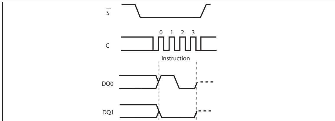
Figure 63. Clear Flag Status Register instruction sequence DIO-SPI
