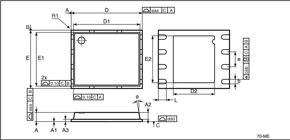
Figure 110. VDFPN8 (MLP8) Very Thin Pitch Dual Flat Package, No Leads, 6x5 mm Drawing
