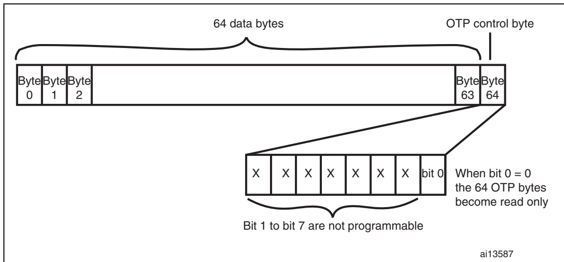
Figure 27. How to permanently lock the OTP bytes
