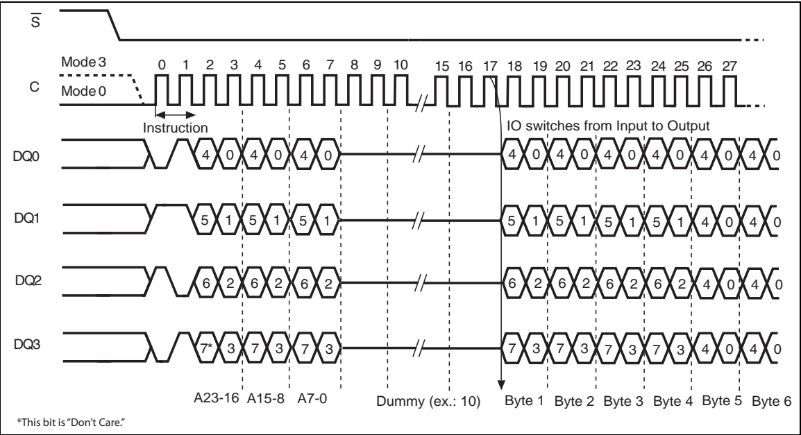
Figure 73. Quad Command Fast Read instruction and data-out sequence QIO-SPI, 6Bh
