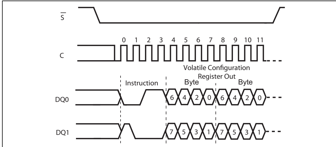
Figure 66. Read Volatile Configuration Register instruction sequence DIO-SPI
