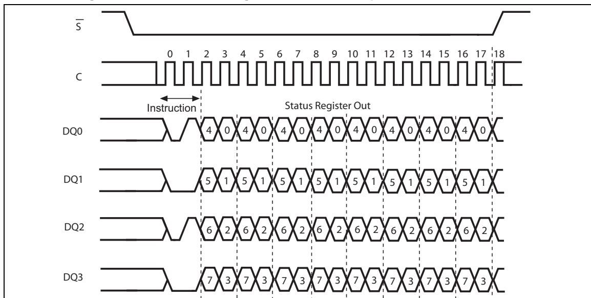
Figure 87. Read Status Register instruction sequence QIO-SPI
