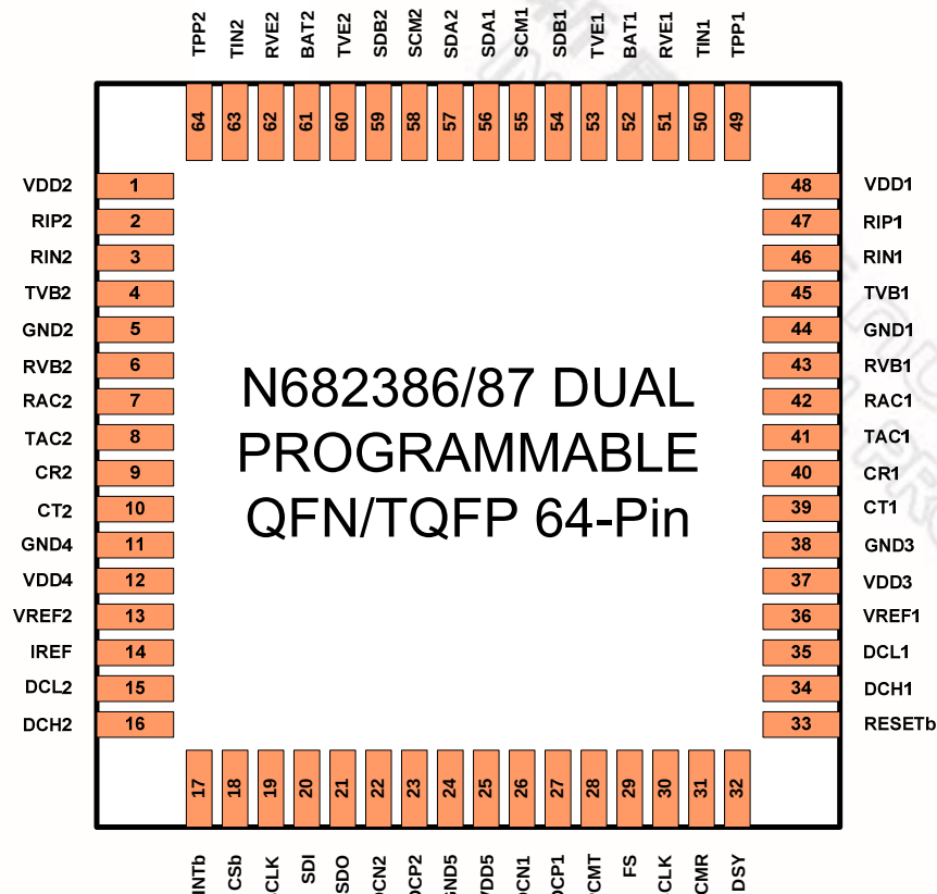
Figure 1: Pin Configuration
