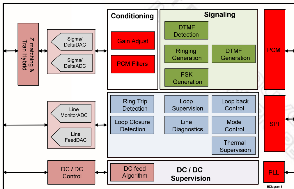
Figure 3: Block Diagram
