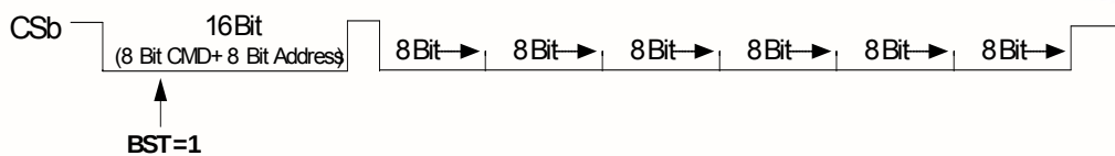
Figure 34: Burst mode operation (BST=1)
