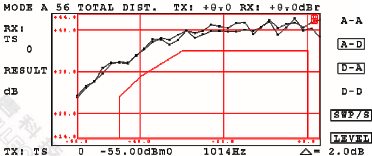
Figure 45: 2-Wire to PCM Signal to Distortion Mask (μ-Law)
