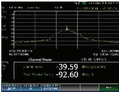
Channel power measurement
