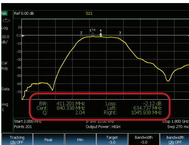
The marker bandwidth/Q factor function simplifies filter testing and tuning.
