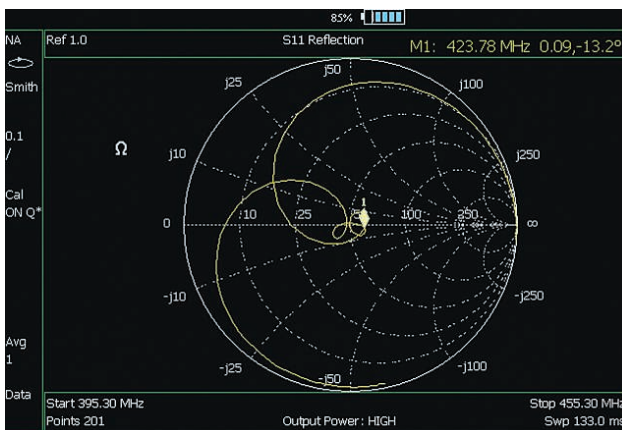
Device input impedance displayed on a Smith chart
