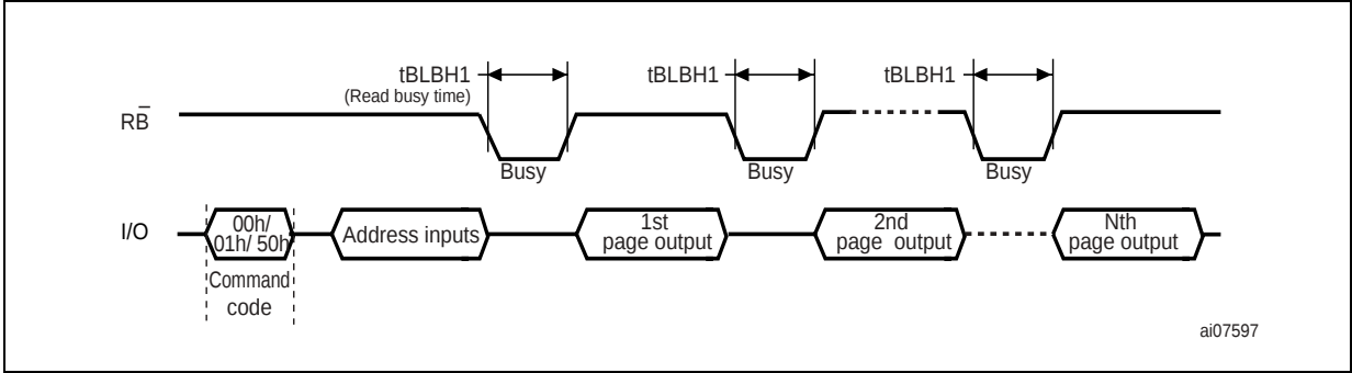
Figure 12. Sequential row read operations
