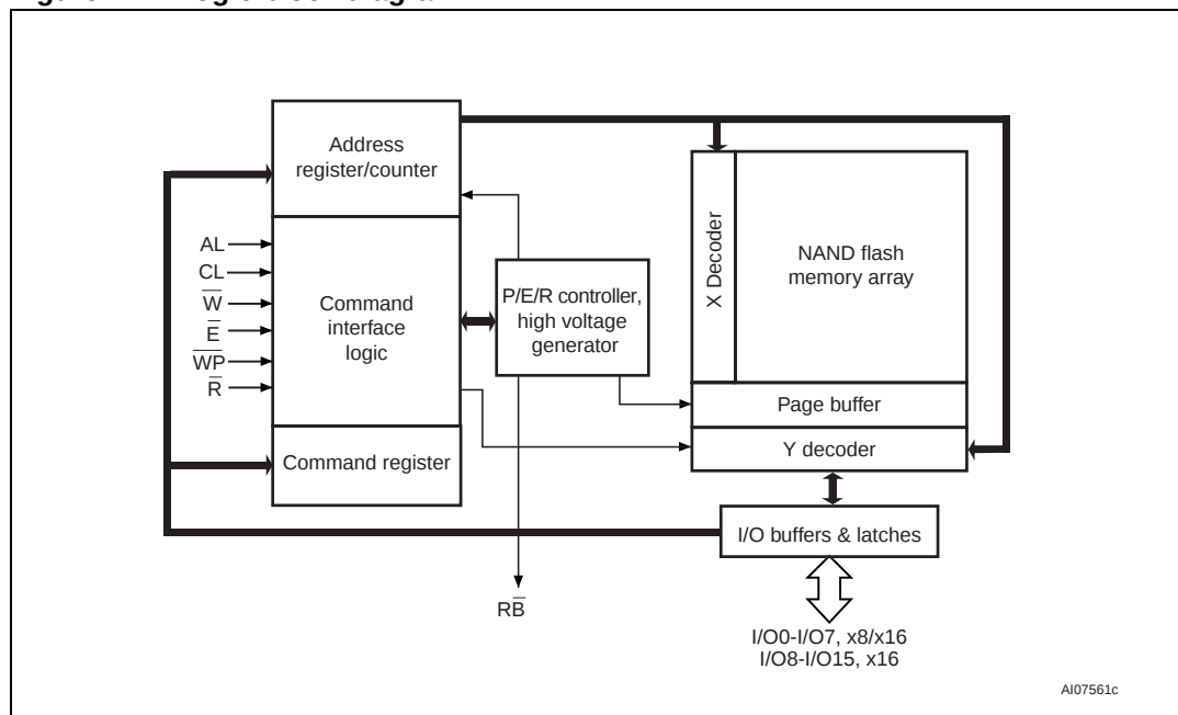
Figure 2. Logic block diagram
