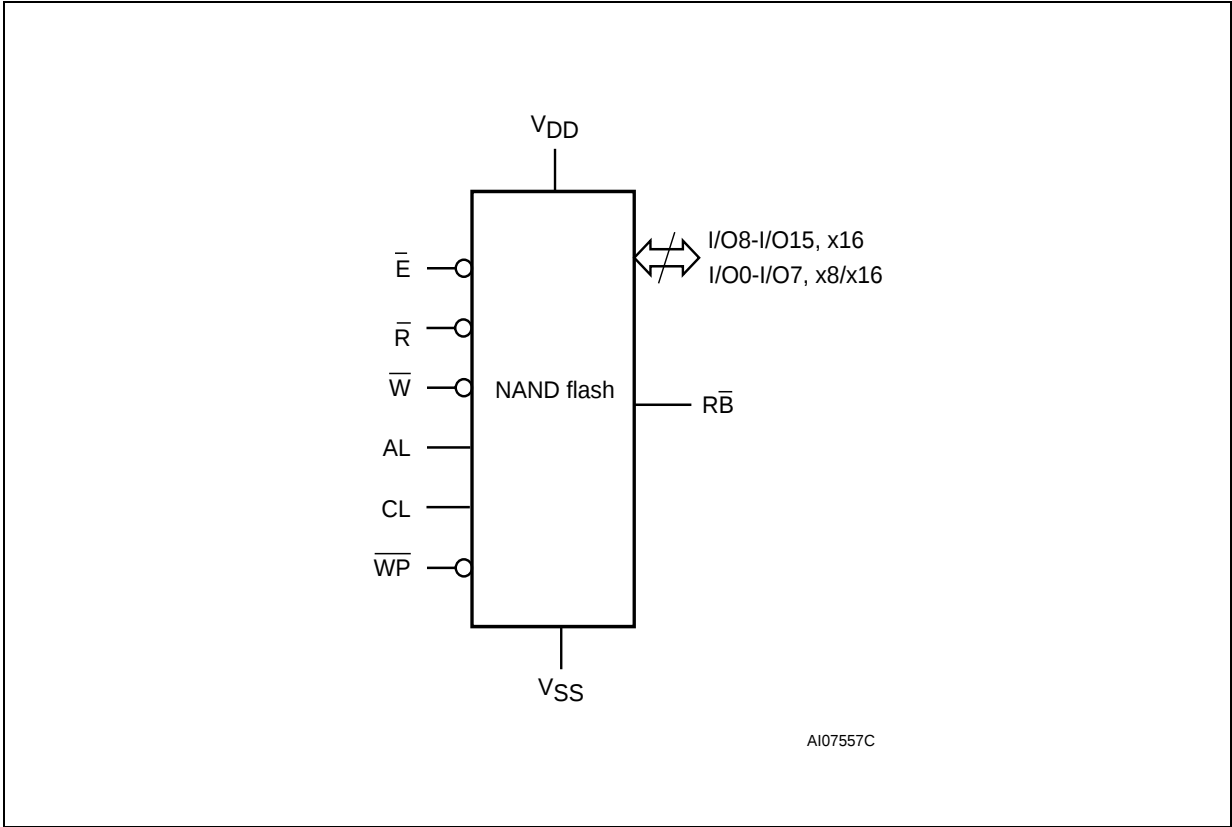
Figure 1. Logic diagram
