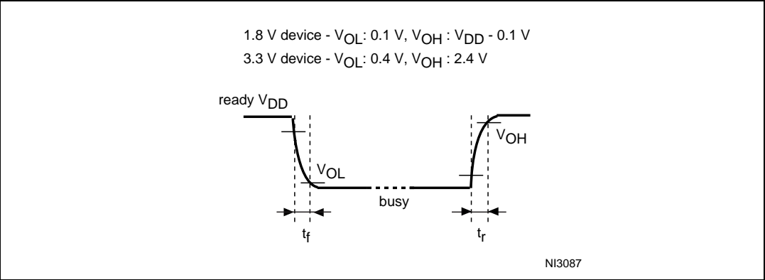
Figure 31. Ready/Busy AC waveform
