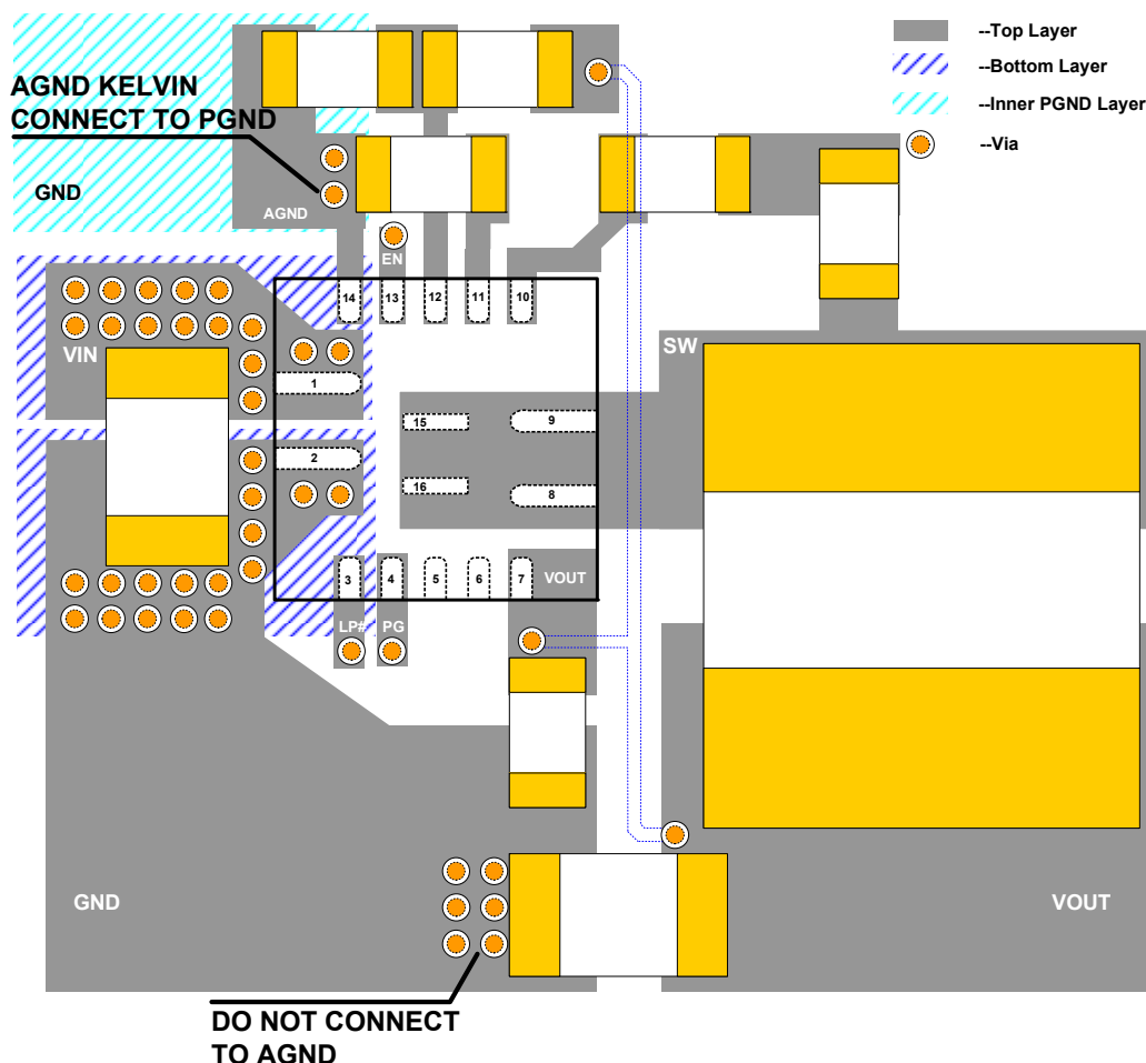
Figure 13—Recommend Layout
