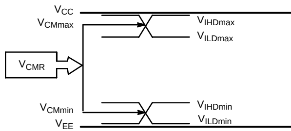
Figure 11. V_{CMR} Diagram
