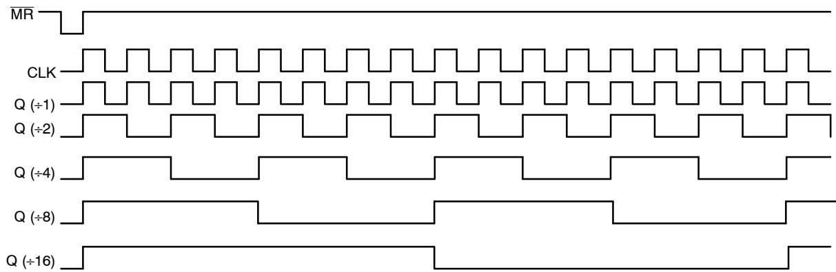
Figure 4. Timing Diagram
