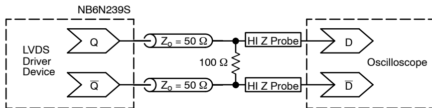
Figure 20. Typical LVDS Termination for Output Driver and Device Evaluation, If Receiver Has On-chip Termination, 100 Ω Resistor is Not Needed
