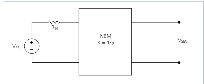
Figure 17 — K = 1/5 NBM with series input resistor
