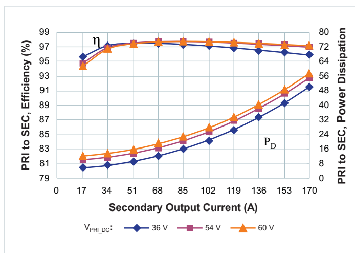
Figure 7 — Efficiency and power dissipation at T_{CASE} = 25^{\circ}\text{C}
