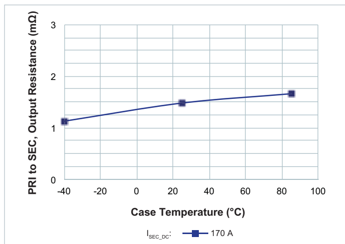
Figure 9 — R_{SEC} vs. temperature; Nominal V_{PRI\_DC} I_{SEC\_DC} = 170\text{ A} at T_{CASE} = 85^{\circ}\text{C}
