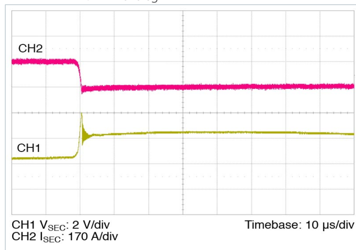
Figure 13 — 170 A – 0 A transient response: C_{PRI\_IN\_EXT} = 300 \mu F, no external C_{SEC\_OUT\_EXT}
