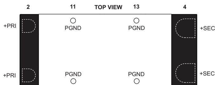
NBM in a 3814 VIA Package - Board (PCB) Mount
