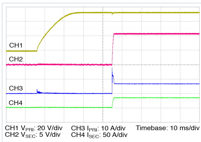
Figure 14 — Forward start up from application of V_{PRI\_DC} = 54 V, 20% I_{OUT} , 100% C_{SEC\_OUT\_EXT}
