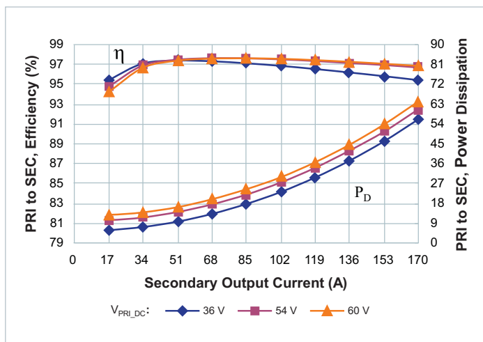
Figure 8 — Efficiency and power dissipation at T_{CASE} = 85^{\circ}\text{C}
