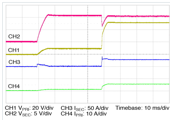
Figure 15 — Reverse start up from application of V_{SEC\_DC} = 10.8 V, 20% I_{PRI\_DG} , 100% C_{PRI\_IN\_EXT}
