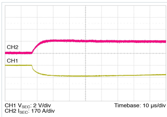
Figure 12 — 0 A– 170 A transient response: C_{PRI\_IN\_EXT} = 300 \mu F, no external C_{SEC\_OUT\_EXT}
