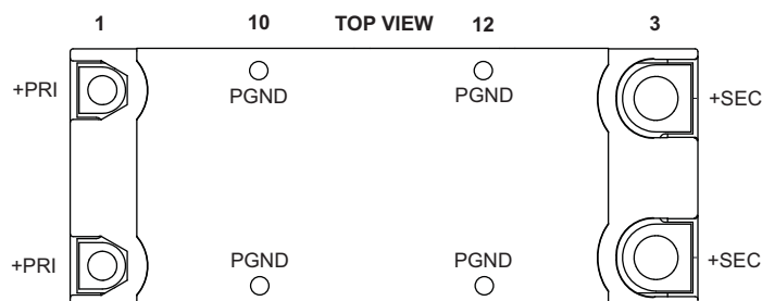
NBM in a 3814 VIA Package - Chassis (Lug) Mount
