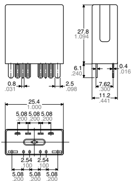
External dimensions
