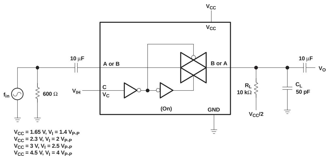
Figure 10. Sine-Wave Distortion
