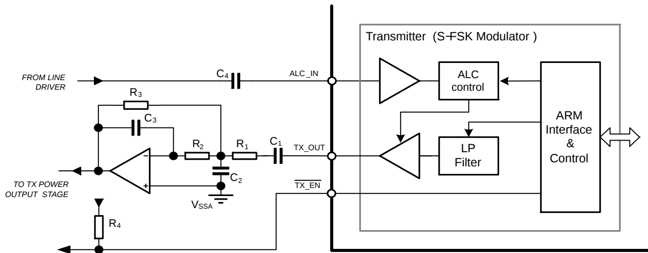
Figure 18. TX_OUT Filter
