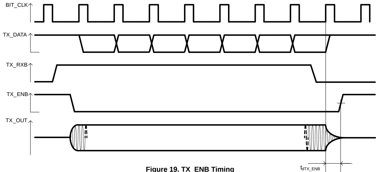
Figure 19. TX_ENB Timing
