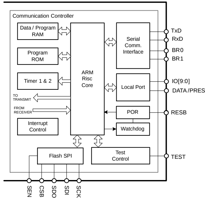
Figure 24. The Communication Controller is Based on a Standard ARM Corex M0 Core
