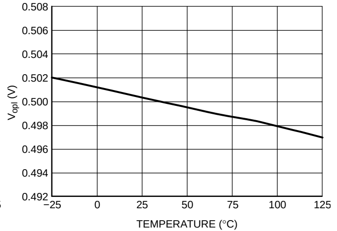
Figure 24. Over Power Limitation Threshold vs. Temperature (NCP1239F)
