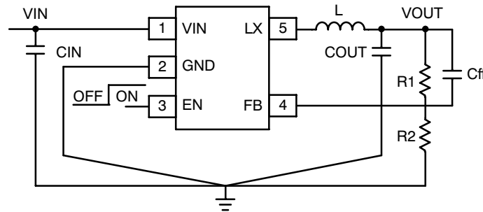
Figure 25. NCP1521 Board Schematic
