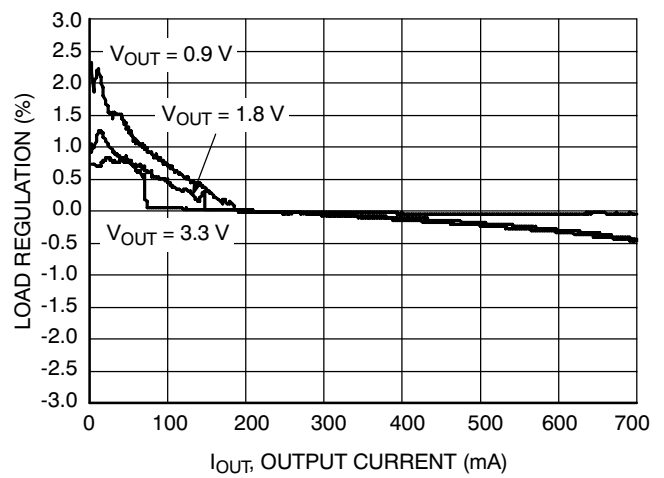
Figure 14. Load Regulation
