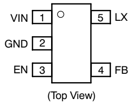
Figure 4. Pin Connections
