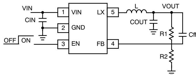
Figure 1. Typical Application
