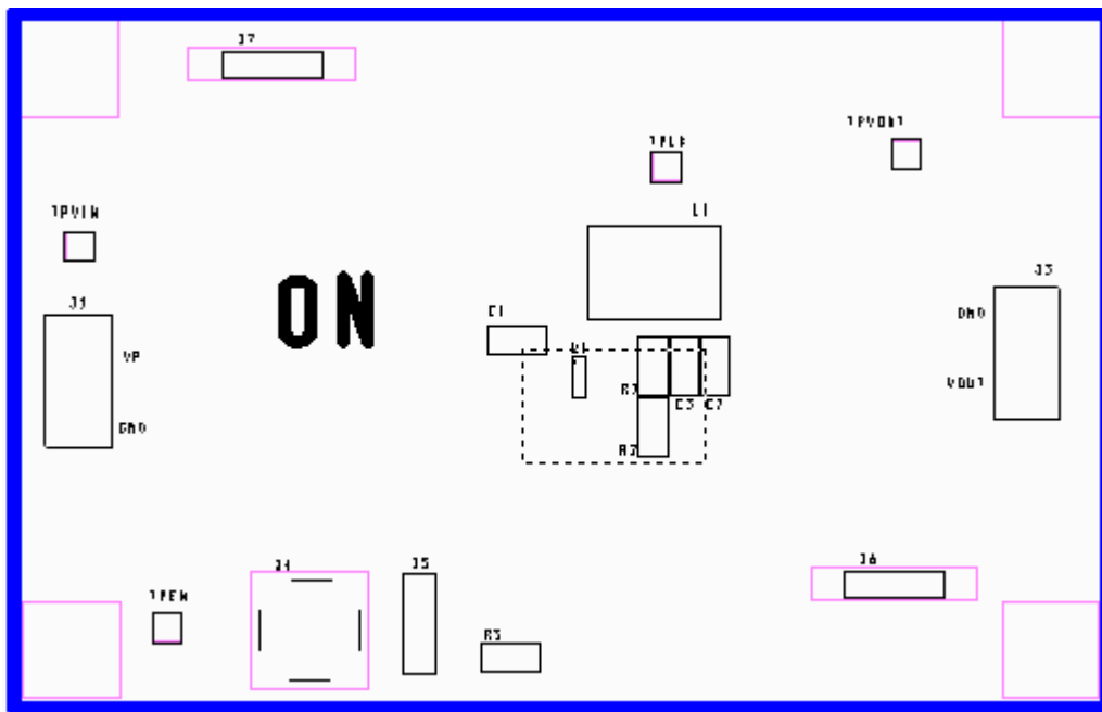
Figure 28. Silkscreen Layer
