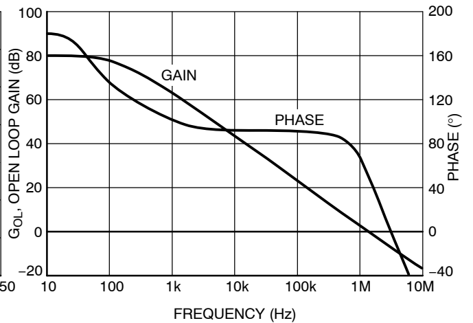
Figure 8. Error Amplifier Open Loop Gain and Phase
