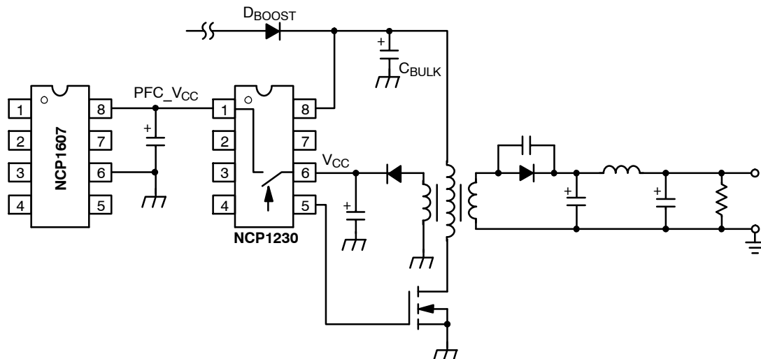
When the PFC pre-converter is loaded by a switch mode power supply (SMPS), then it is often preferable to have the SMPS controller startup first. The SMPS can then supply the NCP1607 V_{CC} directly. Advanced controllers, such as the NCP1230 or NCP1381, can control when to turn on the PFC stage (see Figure 31) leading to optimal system performance. This setup also eliminates the startup resistors and therefore improves the no load power dissipation of the system.
