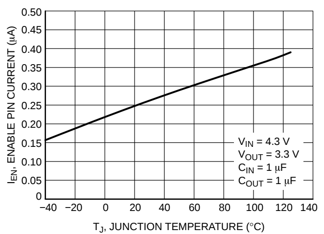
Figure 29. Enable Current vs. Temperature
