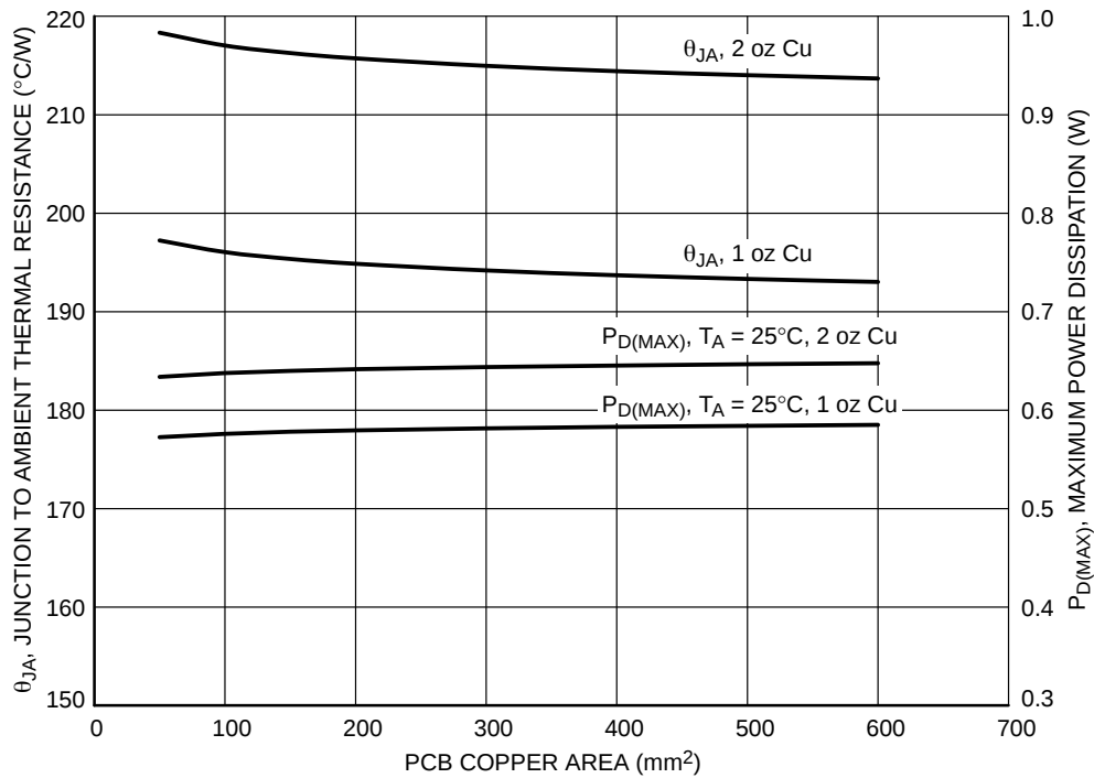
Figure 54. \theta_{JA} and P_{D(MAX)} vs. Copper Area (XDFN44)
